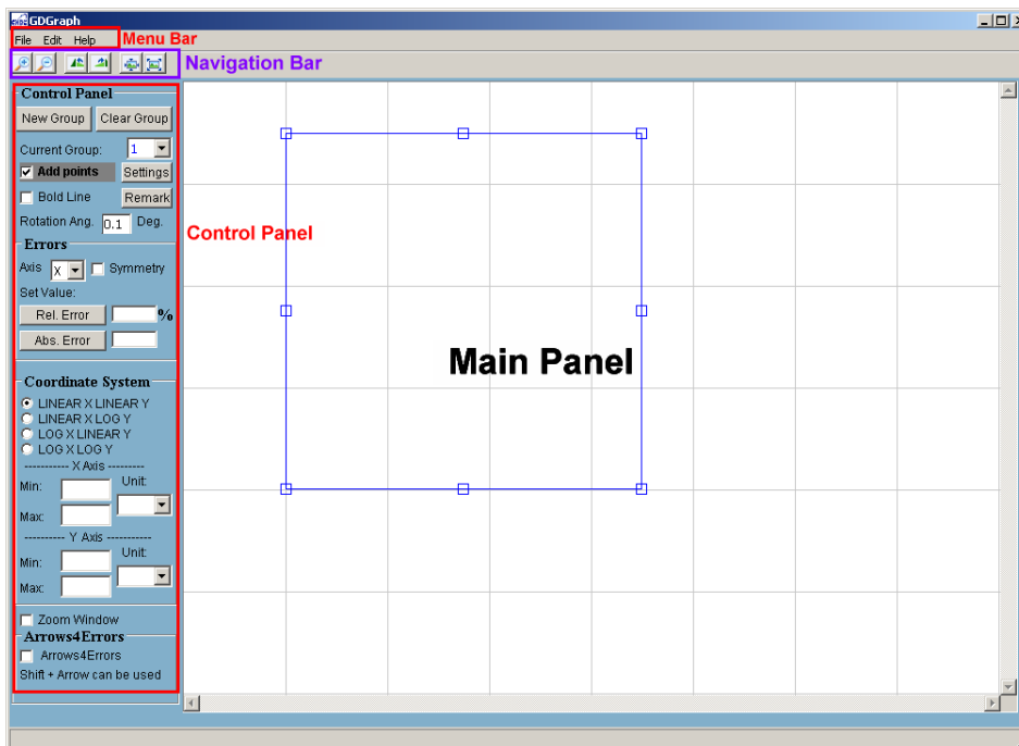
Figure 2.2 Starting-up window of GDGraph5.0. You can select "Load Graph File" or "Load Project File" in "File" menu to load a image file or project file. "Settings" function in the "Edit" menu or "Control Panel".
