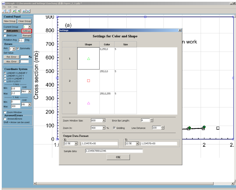
Figure 4.1 Window of "Setting" function. User can set the shape, size and color of data point, output data format, magnifying window, magnified times etc.
