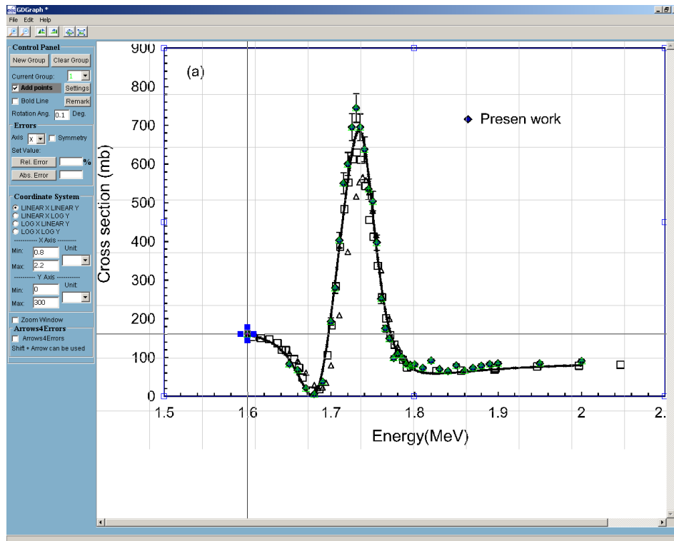
Figure 2.5 Window after reading the data points. The cross lines is help user to confirm the position of data point.
