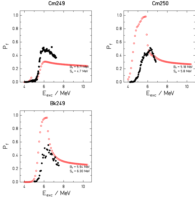
Figure 30: Comparison of the measured fission probabilities (black symbols) with calculations with the GEF code (red symbols).
