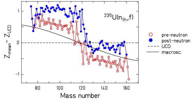
Figure 10: Mean nuclear charge of isobaric chains for different cases for the system ^{235}\text{U}(n_{th}, f) . Dashed line: UCD value. Full line: Macroscopic value at scission. Open symbols: Values before prompt-neutron emission as a function of pre-neutron mass. Full symbols: Values after prompt-neutron emission as a function of post-neutron mass.
