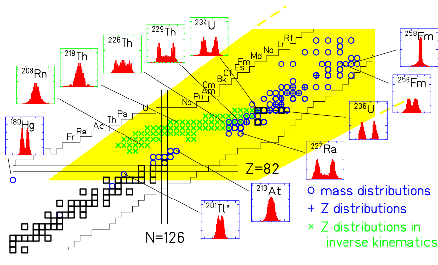
Figure 1: Validity range of the GEF model on a chart of the nuclides, marked in yellow. For a detailed description of the figure see figure 6.
