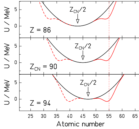
Figure 8: Schematic illustration of the potential energy for mass-asymmetric shape distortions on the fission path, after an idea of M. Itkis et al. [56]. The black curve shows the macroscopic potential that is minimum at symmetry, while the red curve includes the extra binding due to an assumed shell appearing at Z=55 in the heavy fragment. This is not necessarily a proton shell (see text for details).
