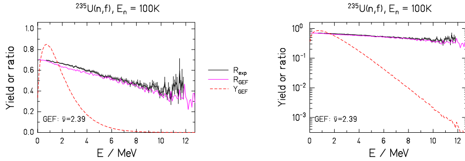
Figure 98: Data from EXFOR dataset 31692006
