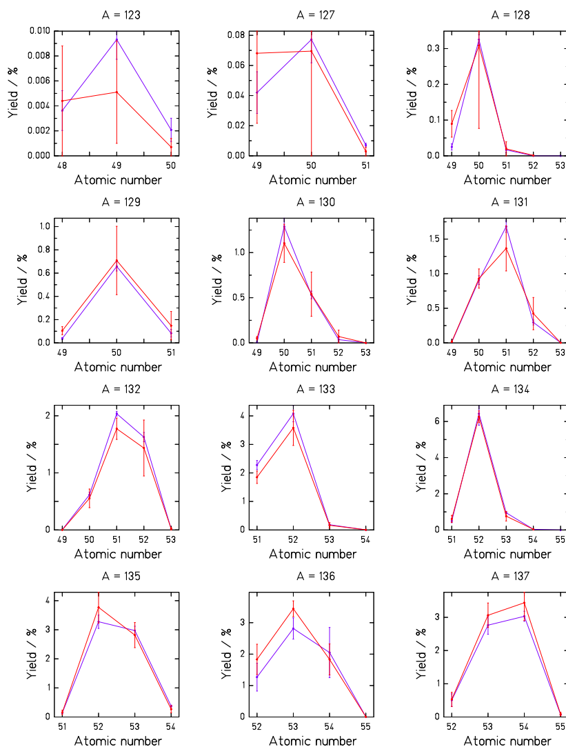
Figure 66: Post-neutron isobaric element distributions in linear scale. The evaluated data [1] (violet symbols) are compared with the results of the GEF code (red symbols). The mass numbers are specified in the figures.
