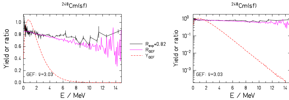
Figure 121: Data from EXFOR dataset 41113004
