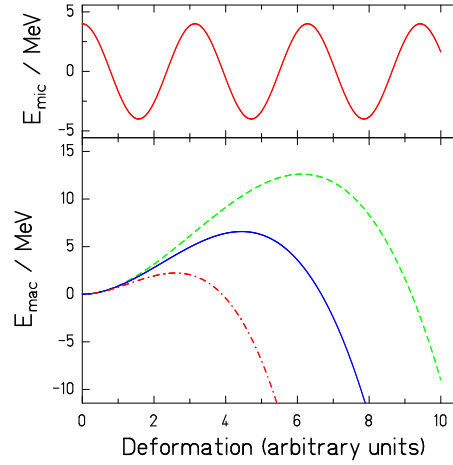
Figure 2: Schematic drawing of the macroscopic and the microscopic potential in fission direction. See text for details.
