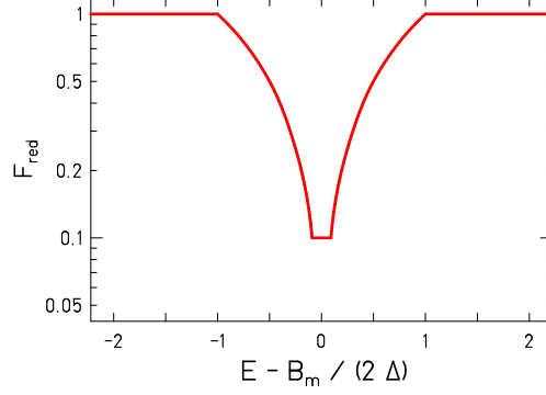
Figure 21: Adapted reduction of the fission-decay width around the fission barrier for even-even nuclei
