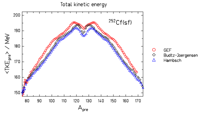
Figure 127: Mean total kinetic energy before evaporation of prompt neutrons as a function of the mass of the fragment for ^{252}\text{Cf(sf)} [190, 172].
