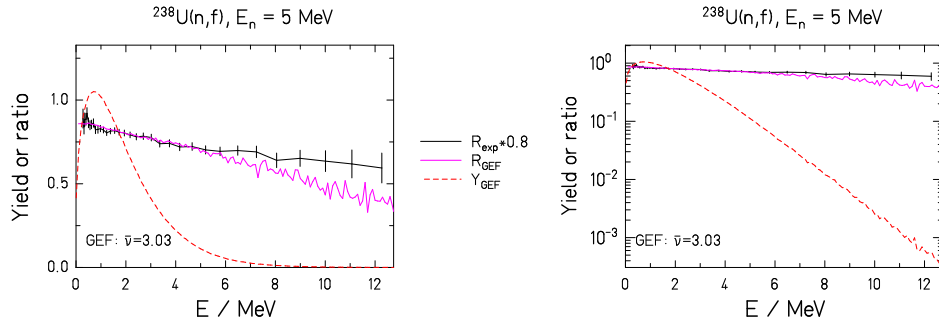
Figure 101: Data from EXFOR dataset 41450003
