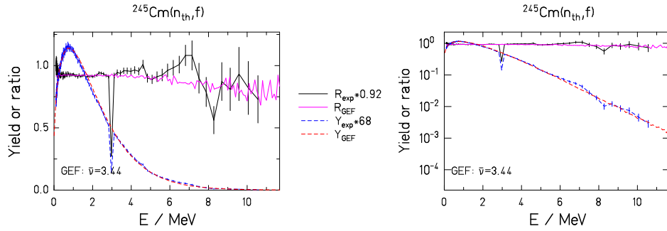
Figure 119: Data from EXFOR dataset 414210091
