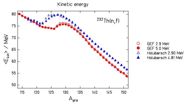
Figure 128: Mean total kinetic energy before evaporation as a function of the mass of the fragment for ^{232}\text{Th(n,f)} [231].
