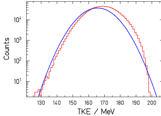
Figure 15: Calculated post-neutron TKE distribution for the system ^{235}\text{U}(n_{th},f) (histogram). The smooth curve shows a fit with a normal distribution.
