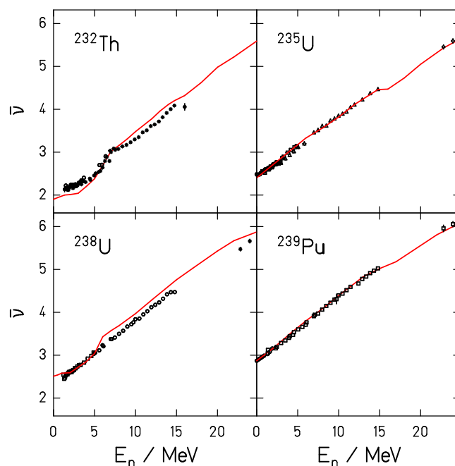
Figure 85: Measured prompt-neutron multiplicity for ^{232}\text{Th}(n,f) , ^{235}\text{U}(n,f) , ^{238}\text{U}(n,f) , and ^{239}\text{Pu}(n,f) (black symbols, different symbols are used for different experiments) as a function of neutron energy (data from ref. [169]) in comparison with the result of the GEF code (red line).
