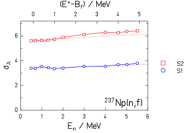
Figure 11: Standard deviation of the mass distribution of the asymmetric fission channels (standard 1 and standard 2) in the fission of ^{237}\text{Np}(n,f) as a function of the neutron energy E_n (lower scale) and the excitation energy above the outer barrier (upper scale). The measured data [66] (symbols) are compared with the calculated widths of the corresponding quantum oscillators (dotted lines).
