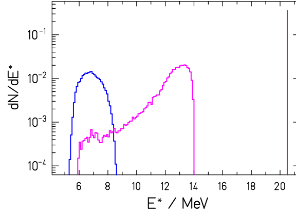
Figure 18: Distribution of excitation energies at fission for the system ^{235}\text{U}(\text{n},\text{f}) at E_n = 14 MeV. The rightmost peak shows events from first-chance fission (fission of ^{236}\text{U} ), the middle curve corresponds to second-chance fission (fission of ^{235}\text{U} ), and the left curve corresponds to third-chance fission (fission of ^{234}\text{U} ).
