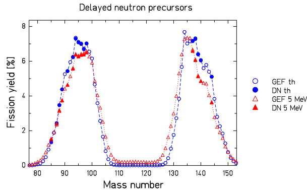
Figure 138: Mass-yield distribution for ^{235}\text{U}(\text{n},\text{f}) at thermal energy and at E_n = 5 MeV calculated with the GEF code. The full points correspond to masses with a main delayed-neutron precursor.
