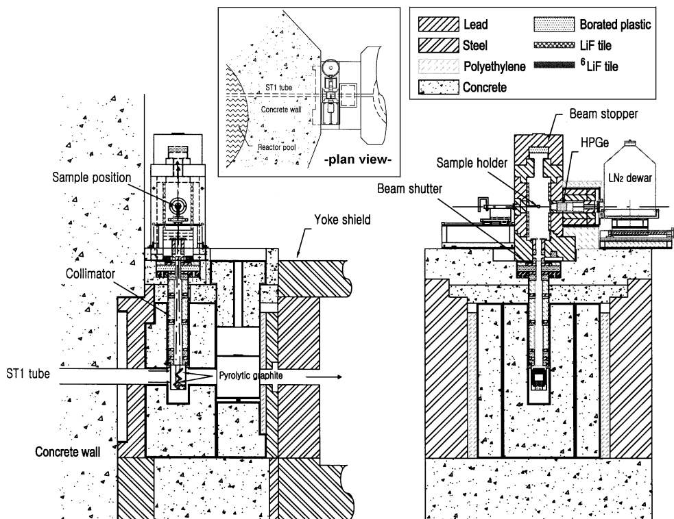
Fig. 1. The PGNA system on the ST1 beam port of HANARO
