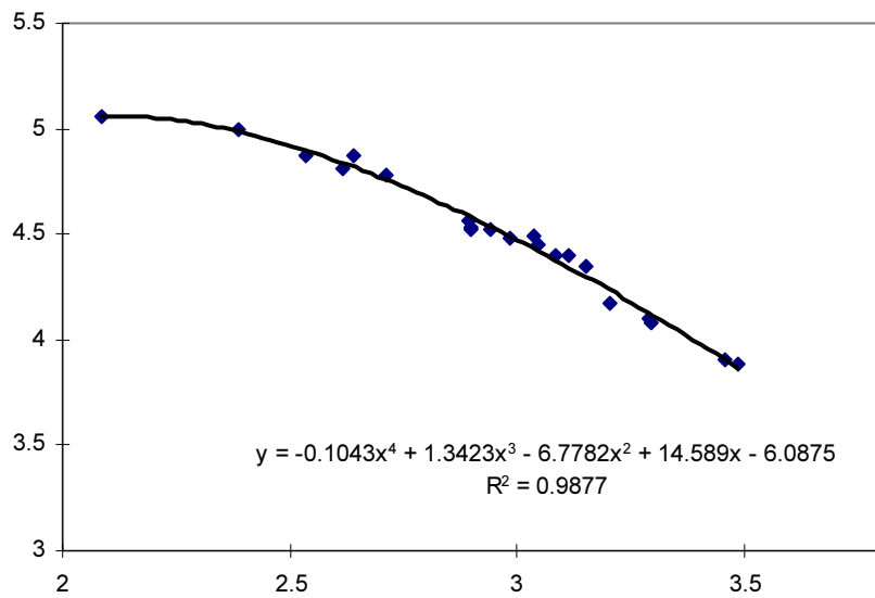
FIG. 2. Relative efficiency curve
