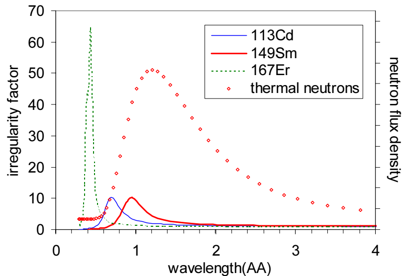
Figure 2. The irregularity factor (the discrepancy from the 1/v -law) of some nuclides as a function of wavelength compared to the thermal neutron spectrum.
