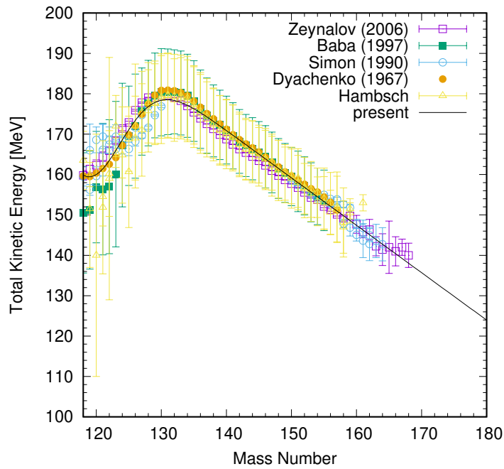
Figure 4: Experimental total kinetic energy as a function of fragment mass together with fitted line.
