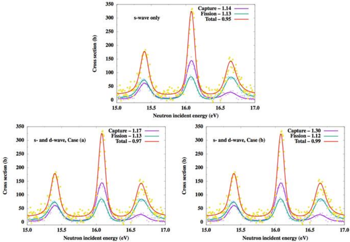
FIG. 1. Example of results obtained on ^{235}\text{U} with the SAMMY code.
