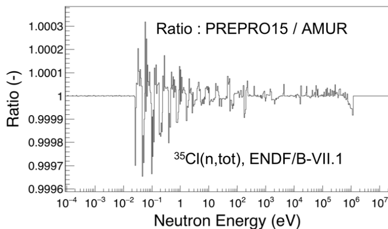
FIG. 1. Ratio of reconstructed cross-sections between PREPRO and AMUR for ^{35}\text{Cl}(n,\text{tot})
