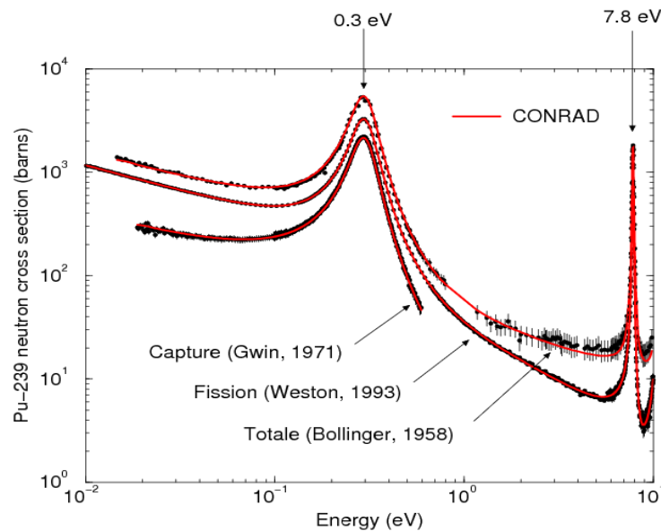
FIG. 1. Example of ^{239}\text{Pu} neutron cross sections calculated with the CONRAD code and compared with EXFOR data.
