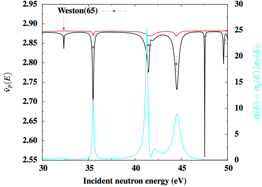
FIG. 2. Prompt neutron multiplicity as a function of the neutron energy.
