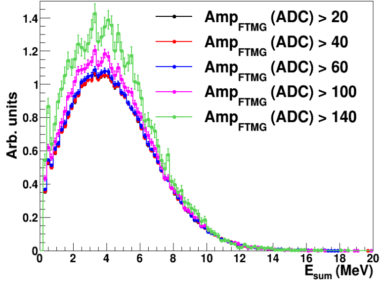
FIG. 1. Total energy deposited in the calorimeter as a function of the threshold set in the MGAS detector.
