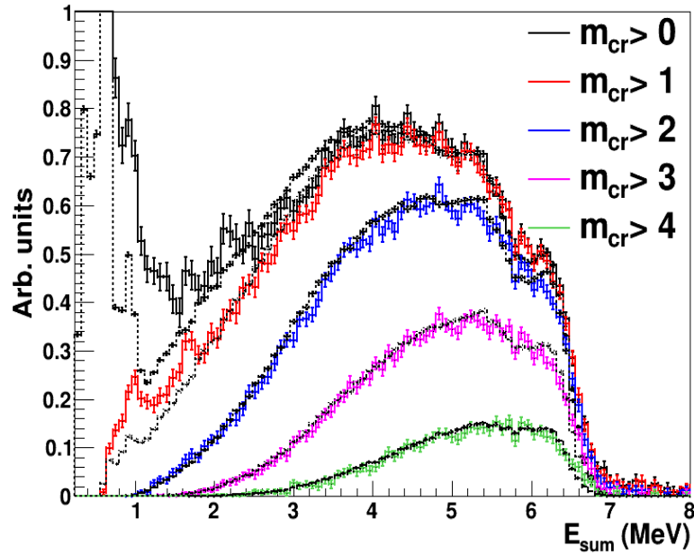
FIG. 2. Coloured histograms: total absorption spectra due to the ^{235}\text{U}(n,\gamma) electromagnetic cascades measured in the TAC as a function of the crystal multiplicity. Solid lines: results from the Monte Carlo simulations for the same conditions on the crystal multiplicity.
