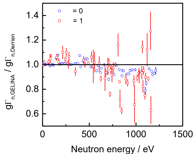
FIG. 1. Ratio of the resonance strengths obtained by Kim et al. and those derived by Derrien et al. as a function of the neutron energy.
