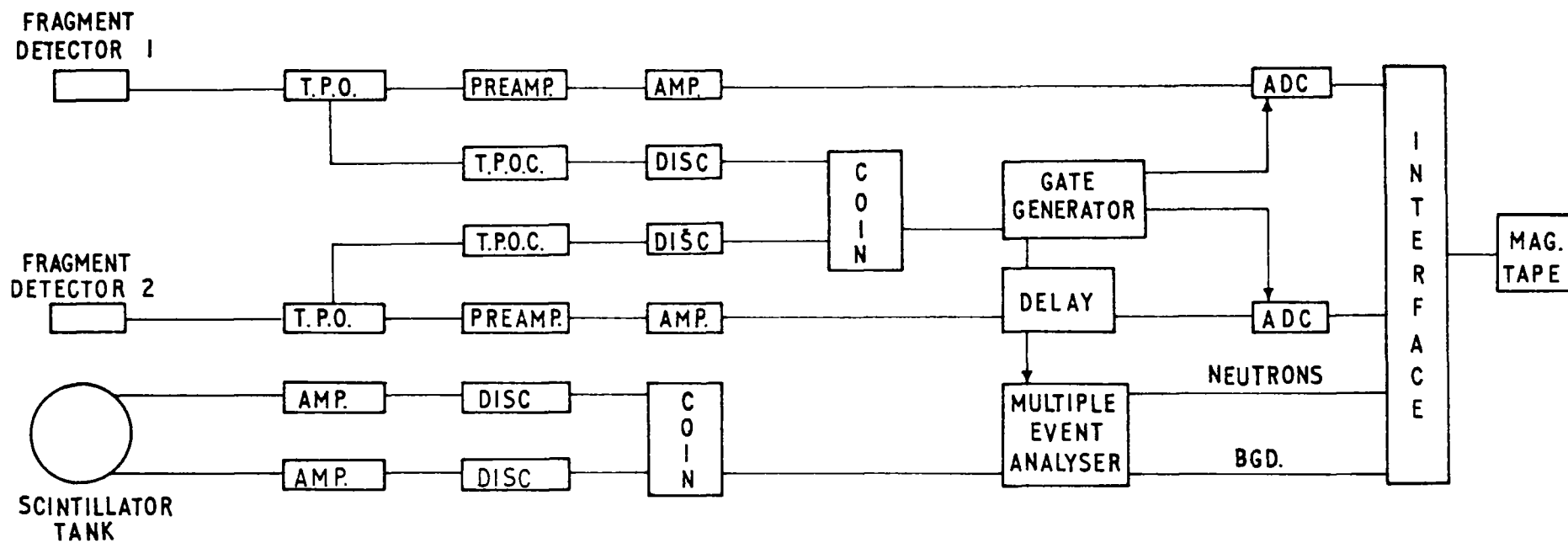
FIGURE 2. BLOCK DIAGRAM OF ELECTRONICS
