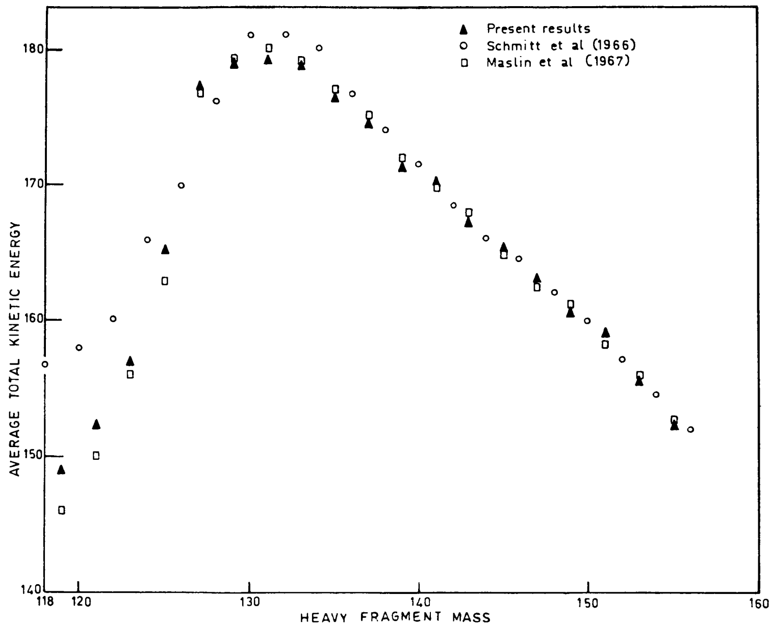
FIGURE 4. MEAN TOTAL FRAGMENT KINETIC ENERGY VERSUS HEAVY FRAGMENT MASS
