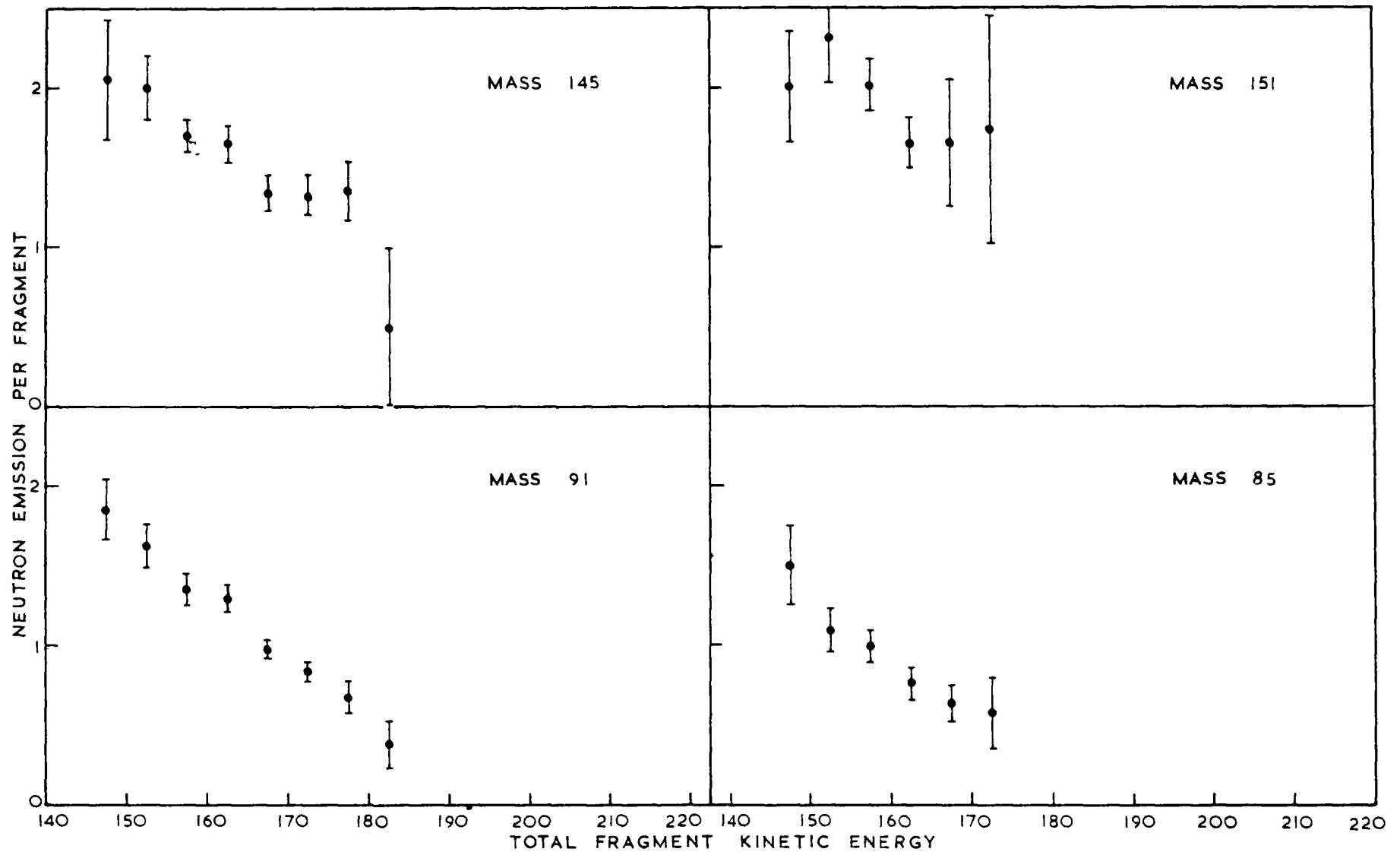
FIGURE 10a. NEUTRON EMISSION PER FRAGMENT VERSUS TOTAL FRAGMENT KINETIC ENERGY FOR EIGHT MASS GROUPS
