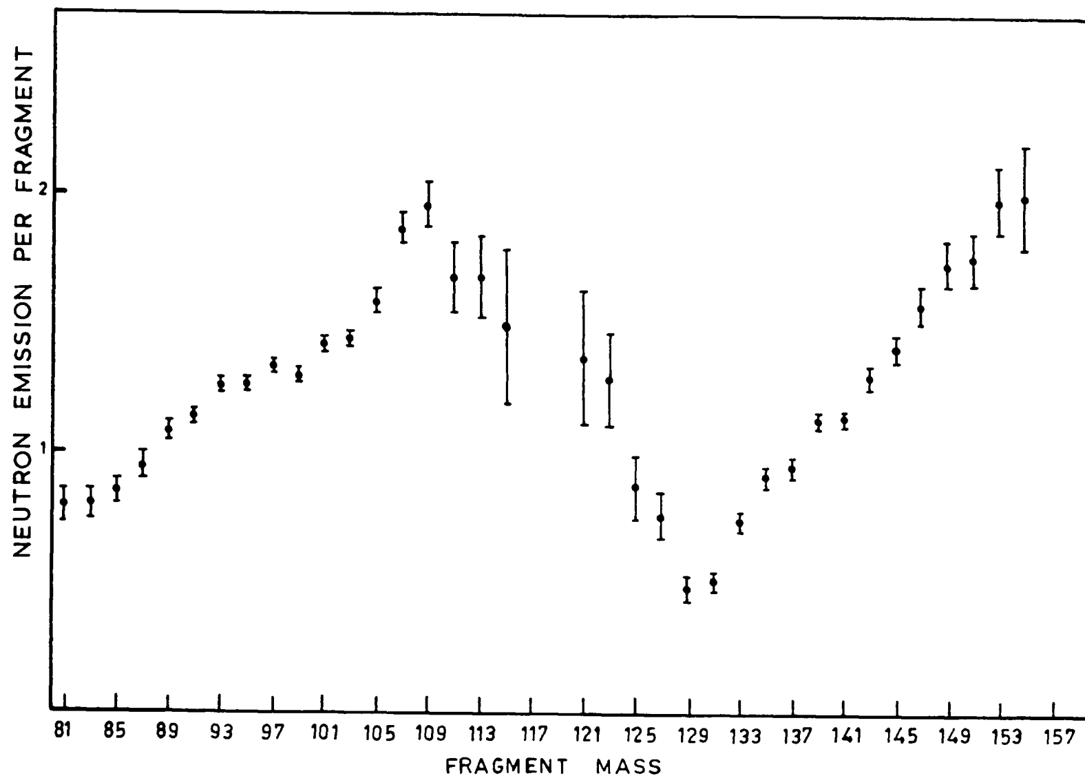
FIGURE 5. NEUTRON EMISSION PER FRAGMENT VERSUS FRAGMENT MASS
