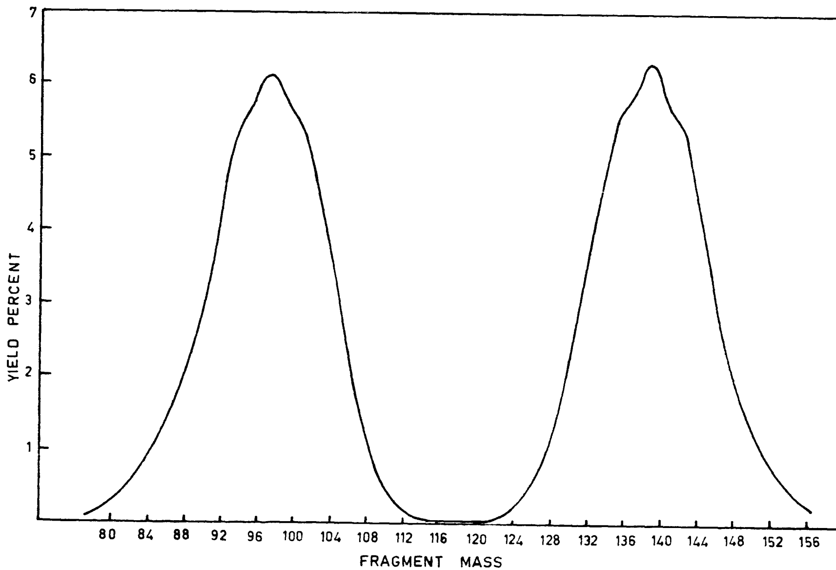
FIGURE 3. PRE-NEUTRON EMISSION MASS DISTRIBUTIONS
