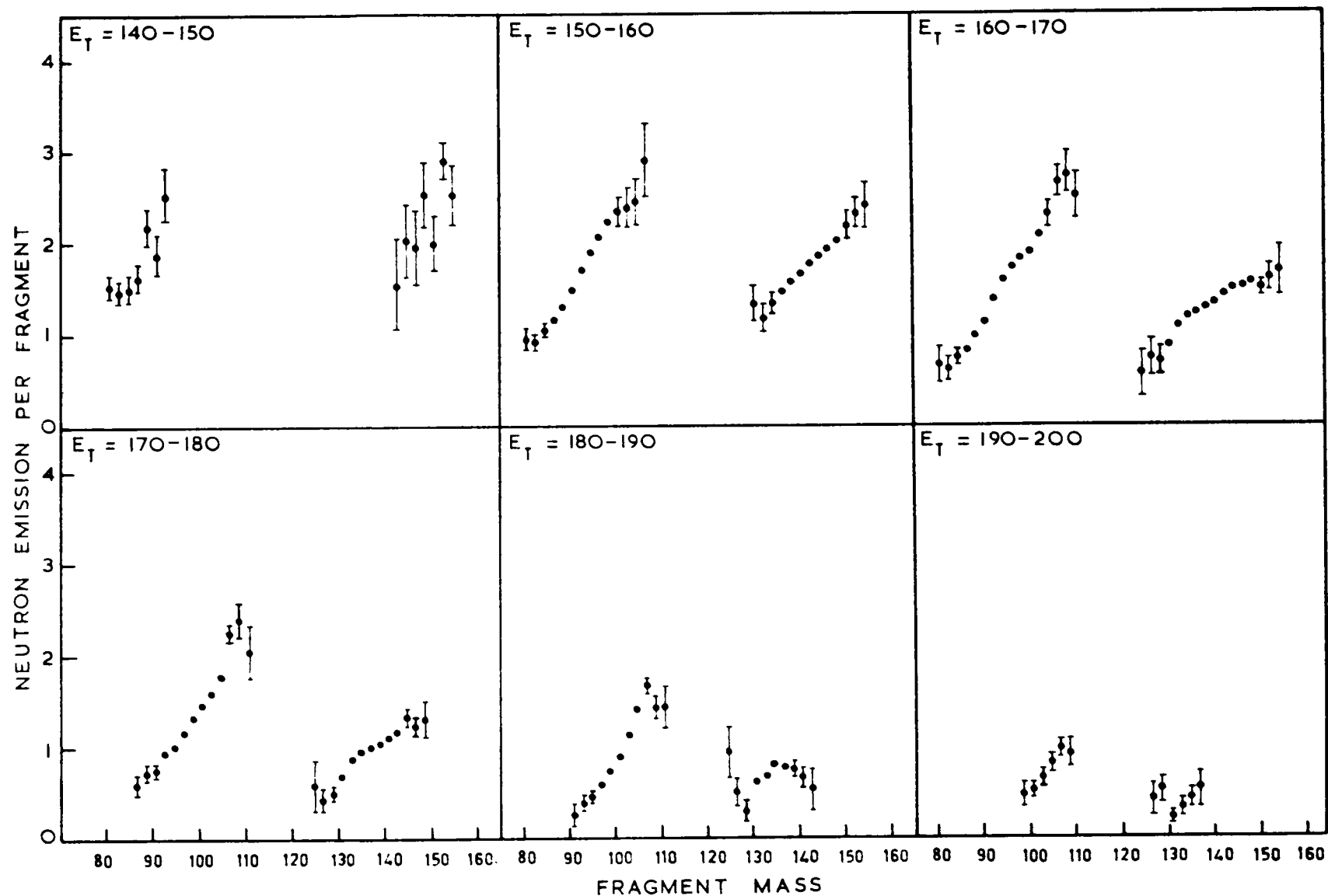
FIGURE 8. NEUTRON EMISSION PER FRAGMENT VERSUS FRAGMENT MASS FOR SIX RANGES OF TOTAL FRAGMENT KINETIC ENERGY
