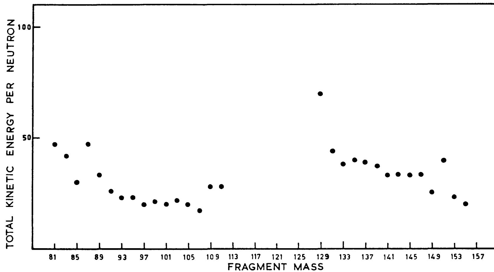
FIGURE 11. THE SLOPE \frac{dE}{d\gamma} VERSUS FRAGMENT MASS
