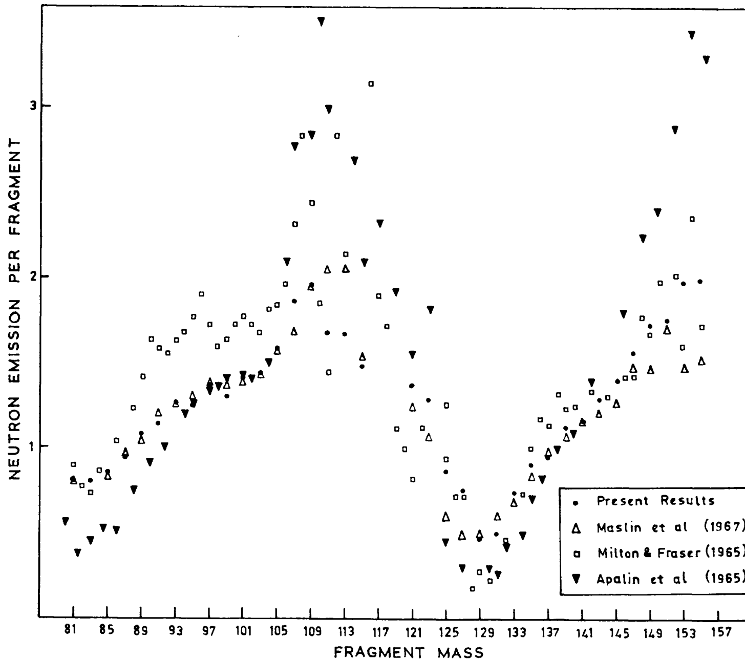
FIGURE 7. COMPARISON OF PRESENT NEUTRON EMISSION DATA WITH PREVIOUS DIRECT NEUTRON COUNTING DATA
