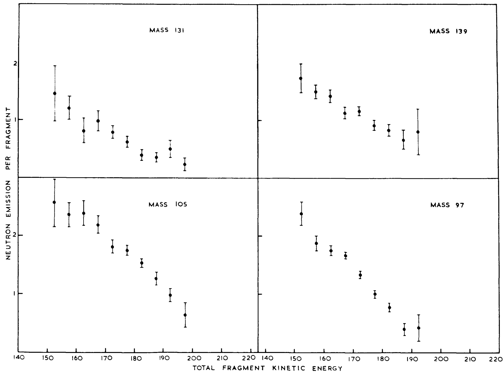
FIGURE 10b. NEUTRON EMISSION PER FRAGMENT VERSUS TOTAL FRAGMENT KINETIC ENERGY FOR EIGHT MASS GROUPS
