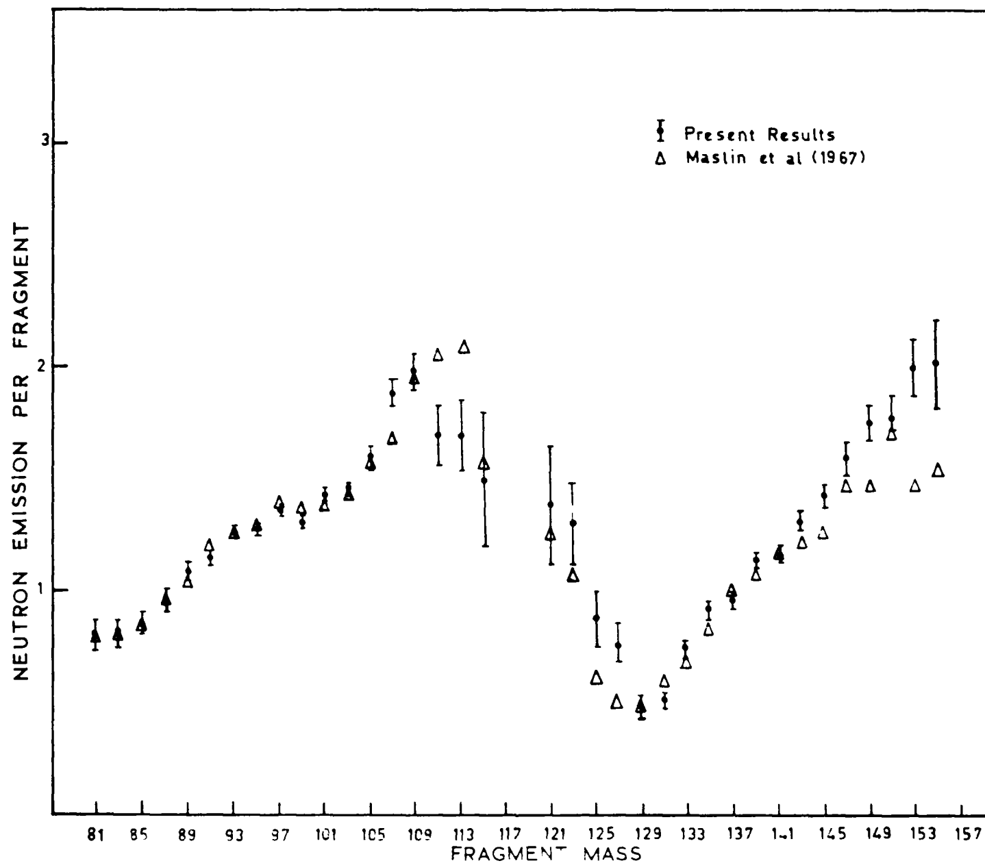
FIGURE 6. COMPARISON OF PRESENT DATA WITH THOSE OF MASLIN ET AL (1967)
