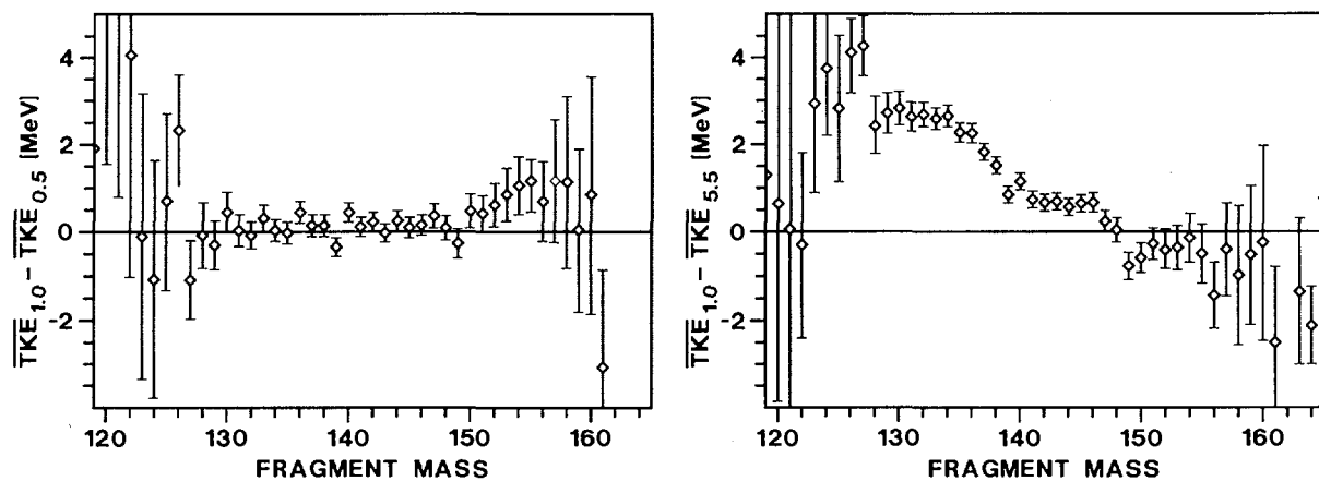
Fig. 9. Difference of the \overline{TKE} as function of the heavy fragment mass at E_n = 1.0 MeV and E_n = 0.5 MeV (left part) and at E_n = 1.0 MeV and E_n = 5.5 MeV (right part)
