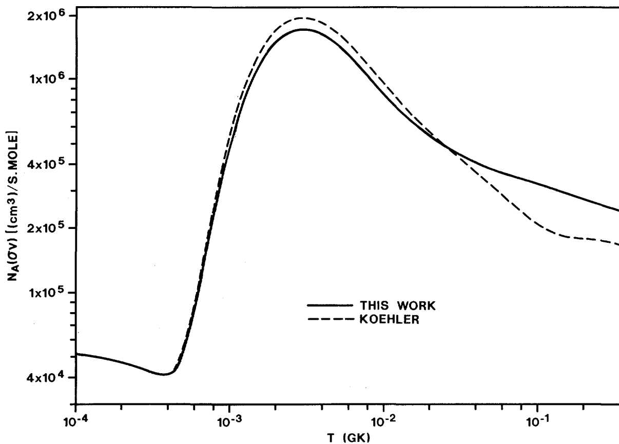
Fig. 28. Comparison of the stellar reaction rates calculated from Koehler's renormalized data and the present work, as a function of the stellar temperature
