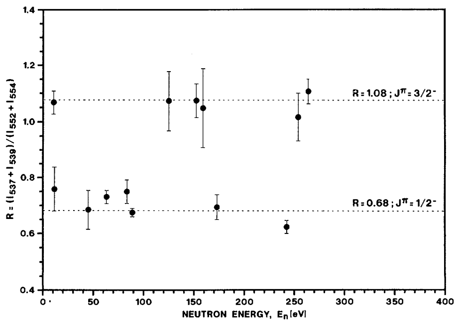
Fig. 21. The ratios R between the sums of the intensities of the relevant lines plotted versus the resonance energy for 14 p -waves
