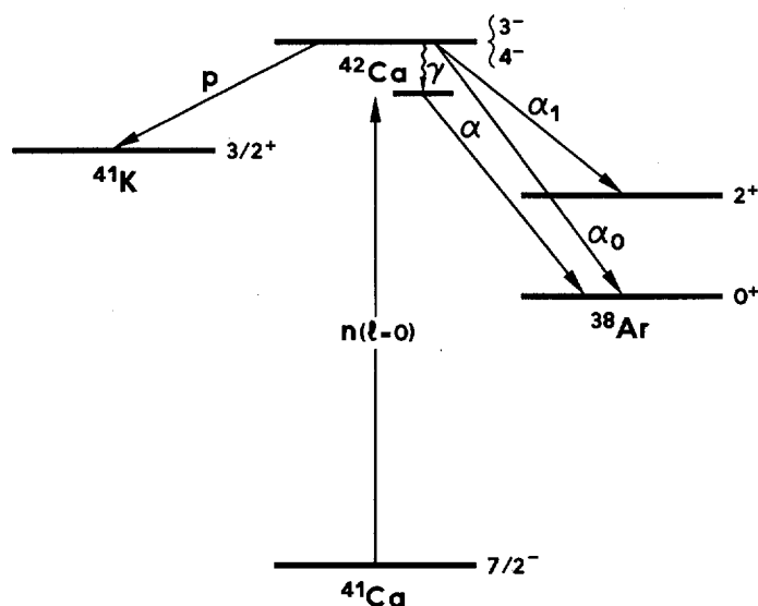
Fig. 30. Schematic representation of the proton and \alpha -decays of the compound nucleus ^{42}\text{Ca} formed after (s-wave) neutron capture in ^{41}\text{Ca}
