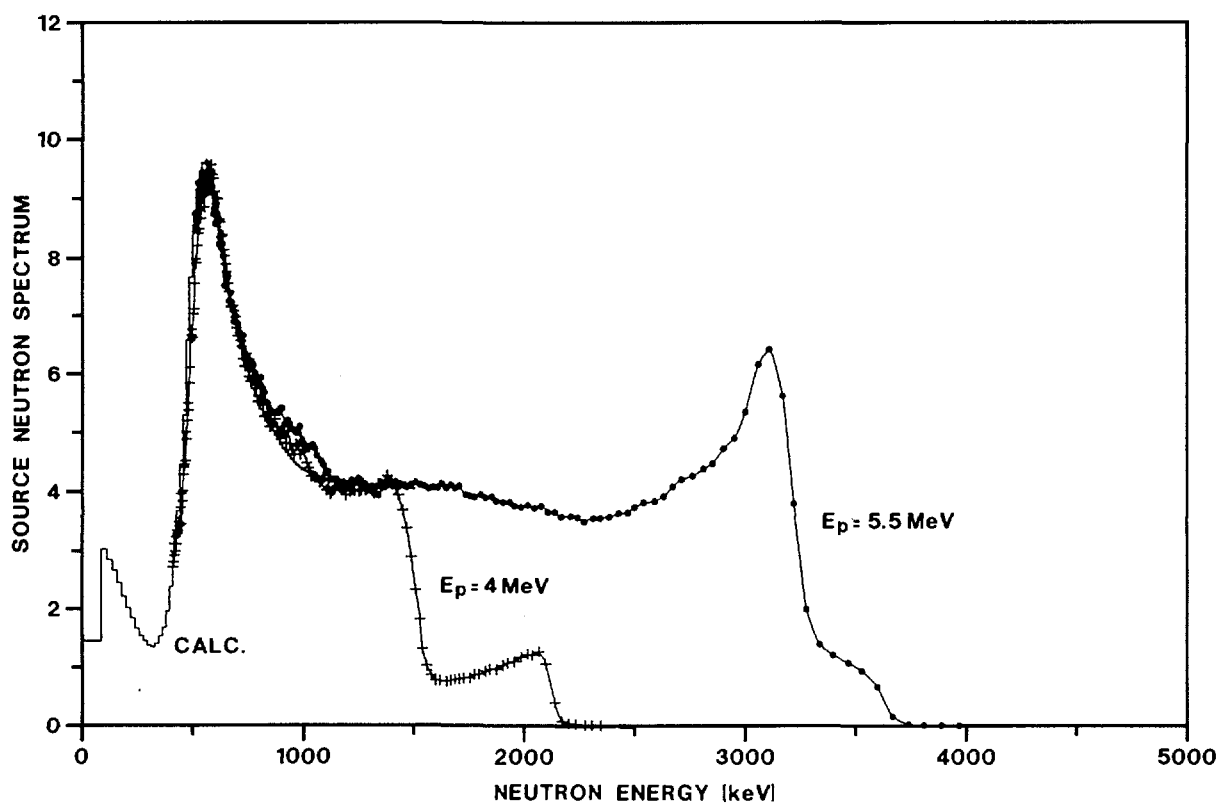
Fig. 15. Thick target neutron energy spectra for E_p = 4 MeV and 5.5 MeV. The ordinate is in arbitrary units
