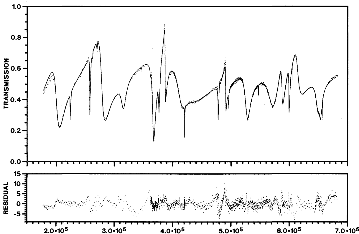
Fig. 16. REFIT fit (continuous line) to the neutron transmission through 0.19293 at/b of aluminium in the energy range 180 to 680 keV
