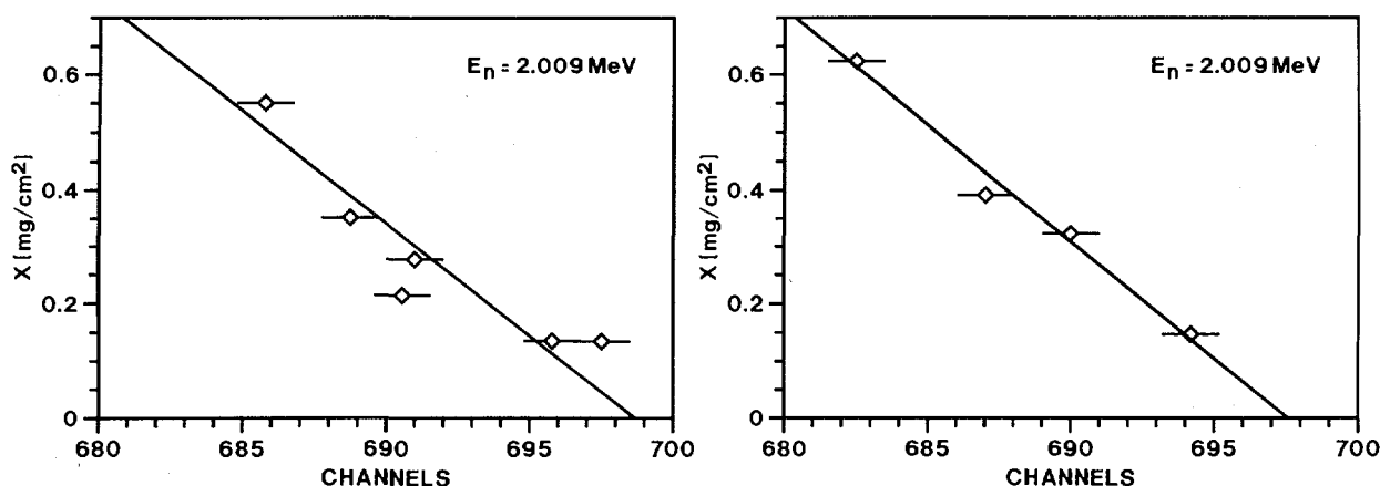
Fig. 2. Sample thickness versus channel number at half height of the proton recoil distribution, left part: octacosanol, right part: tristearin. Straight line fit to get the stopping power at about 2 MeV incident neutron energy
