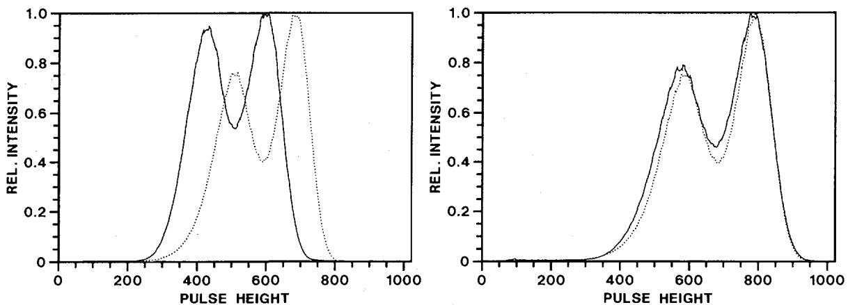
Fig. 5. Comparison of raw spectra measured at different pressure. Left part: methane 1.2 \cdot 10^5 Pa (solid line), 0.6 \cdot 10^5 Pa (dotted line) and right part: 90 % Ar + 10 % CH 4 1.2 \cdot 10^5 Pa (solid line), 0.6 \cdot 10^5 Pa (dotted line)
