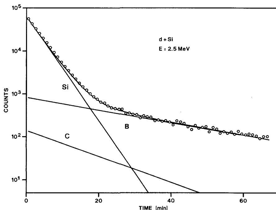
Fig. 37. Decay curve from a silicon (Si) sample containing boron (B) and carbon (C) after irradiation with 2.5 MeV deuterons and its decomposition. The circles are measured data, the solid line through them is the fitting function (sum of three exponentials, also shown as solid lines)
