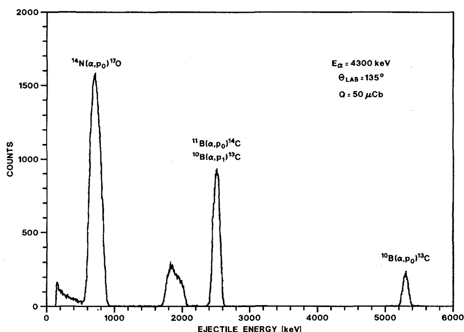
Fig. 34. Energy spectrum from the \alpha -particle bombardment of a BN-coating on a stainless steel substrate
