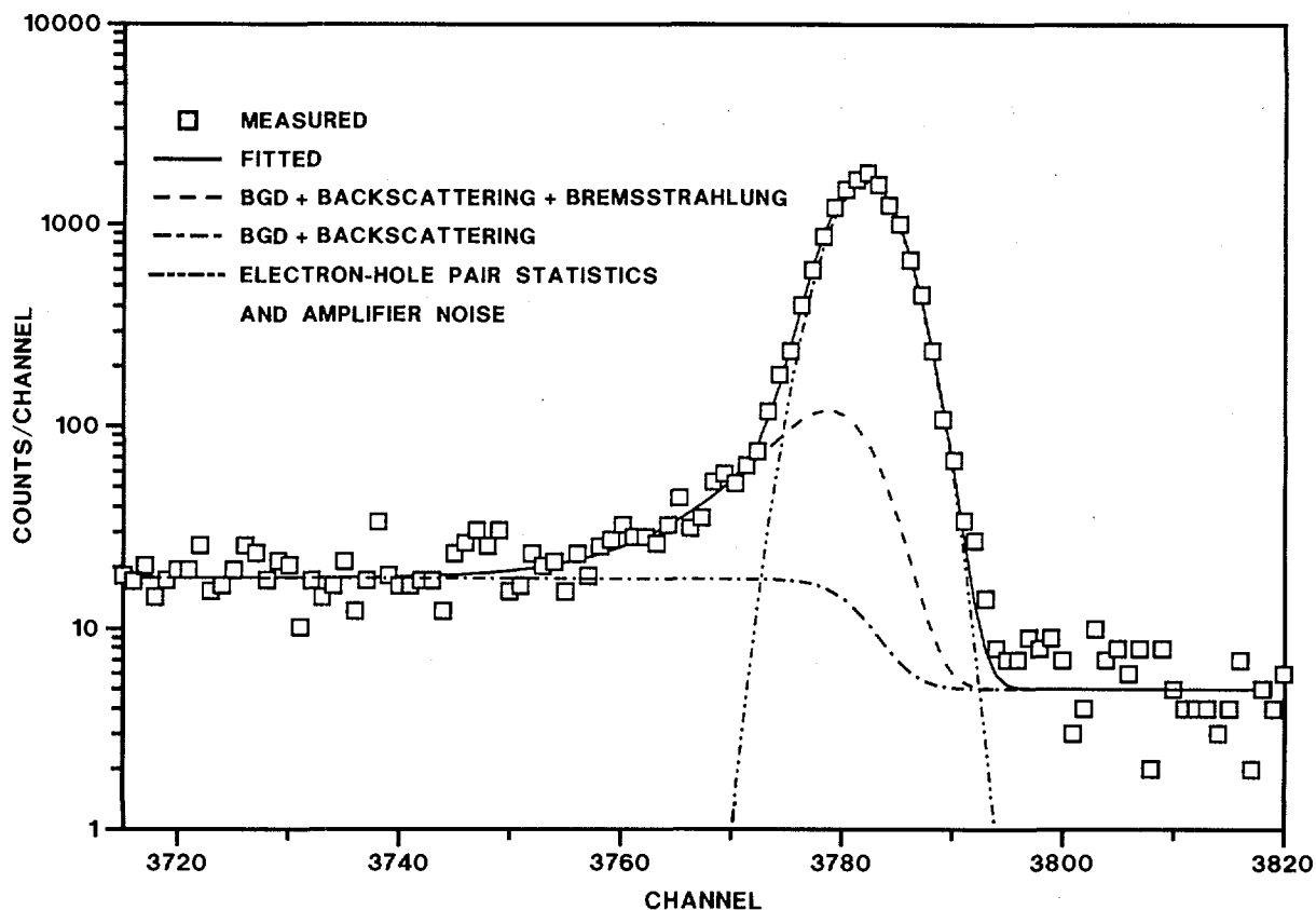
Fig. 31. Response function of a 50 mm 2 PIPS detector for K-shell conversion electrons from the 207 Bi decay at 975.6 keV
