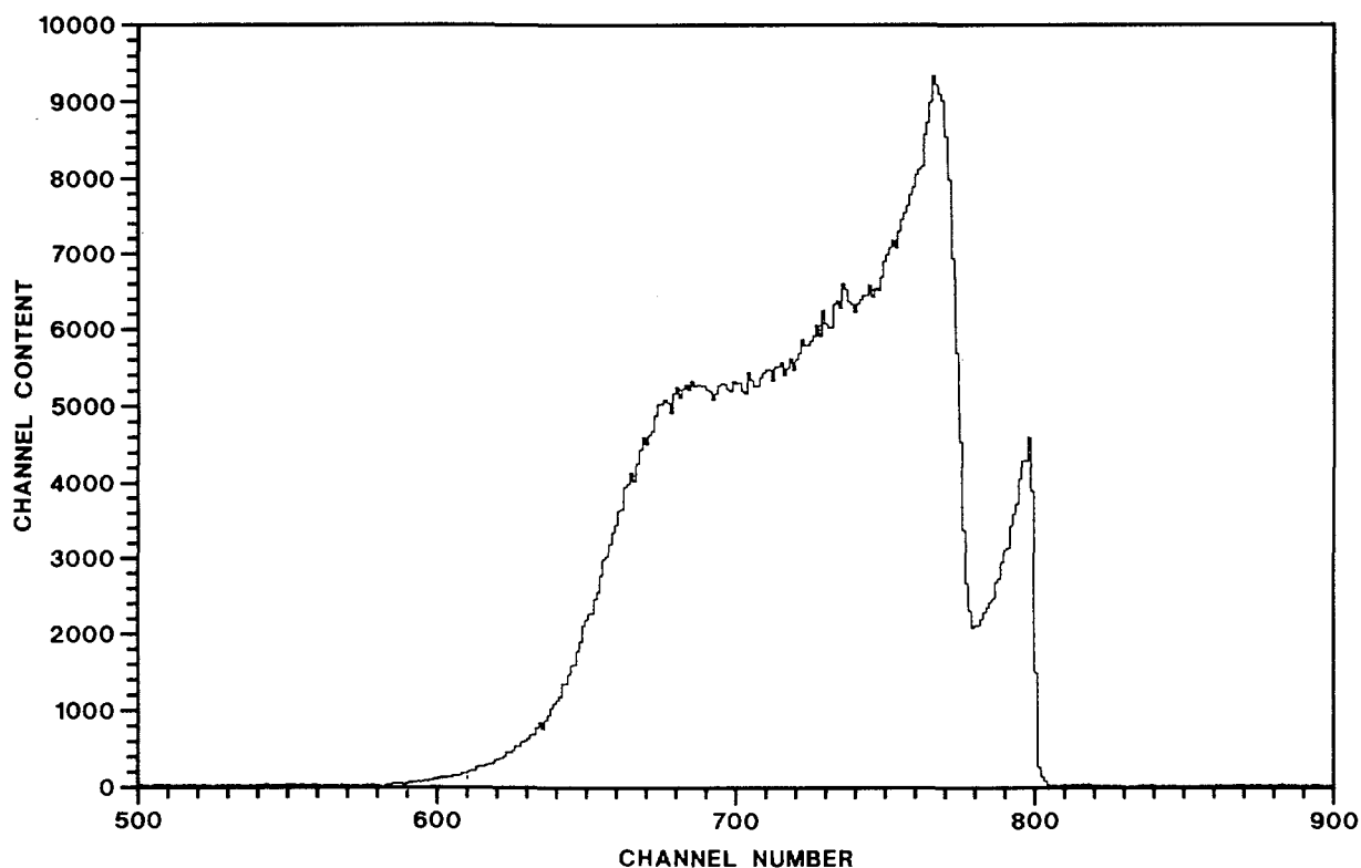
Fig. 14. Neutron time-of-flight spectrum for E_p = 4 MeV, 4.318 m flight path and 1.56 ns time channel width (large time-of-flight at small channel number)
