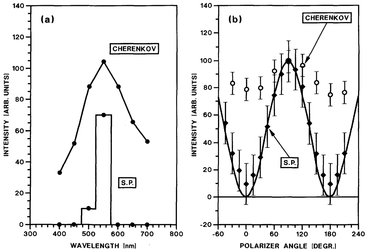
Fig. 33. Smith-Purcell radiation generated by a 110 MeV electron beam. (a) Spectral distribution measured with narrow-band filters. Predicted wavelength of SP radiation: (559 \pm 10) nm. (b) Measurement of the linear polarization. Solid line: theoretical prediction for a pure H-polarized radiation. Values normalized at 90^\circ
