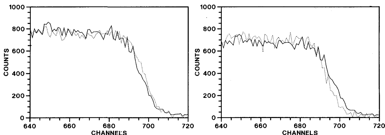
Fig. 1. Comparison of the proton recoil spectra for about 2 MeV incident neutron energy and octacosanol sample thicknesses of 137 \mu\text{g}/\text{cm}^2 (solid line) and 136 \mu\text{g}/\text{cm}^2 (dotted line) (left part) and octacosanol sample of 137 \mu\text{g}/\text{cm}^2 (solid line) and tristearin sample of 148 \mu\text{g}/\text{cm}^2 (dotted line) (right part)
