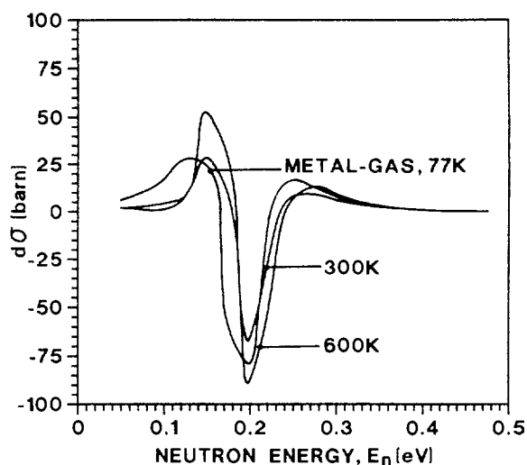
Fig. 27. Differences in the capture cross-section in the vicinity of the 0.18 eV resonance of ^{113}\text{Cd} for the Doppler broadening in Cd metal and a gas, with temperatures 77, 300 and 600K
