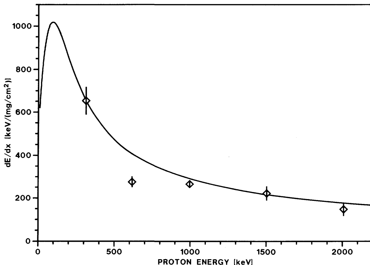
Fig. 3. Stopping power values of ref. (1) (solid line) compared to the measured ones of octacosanol
