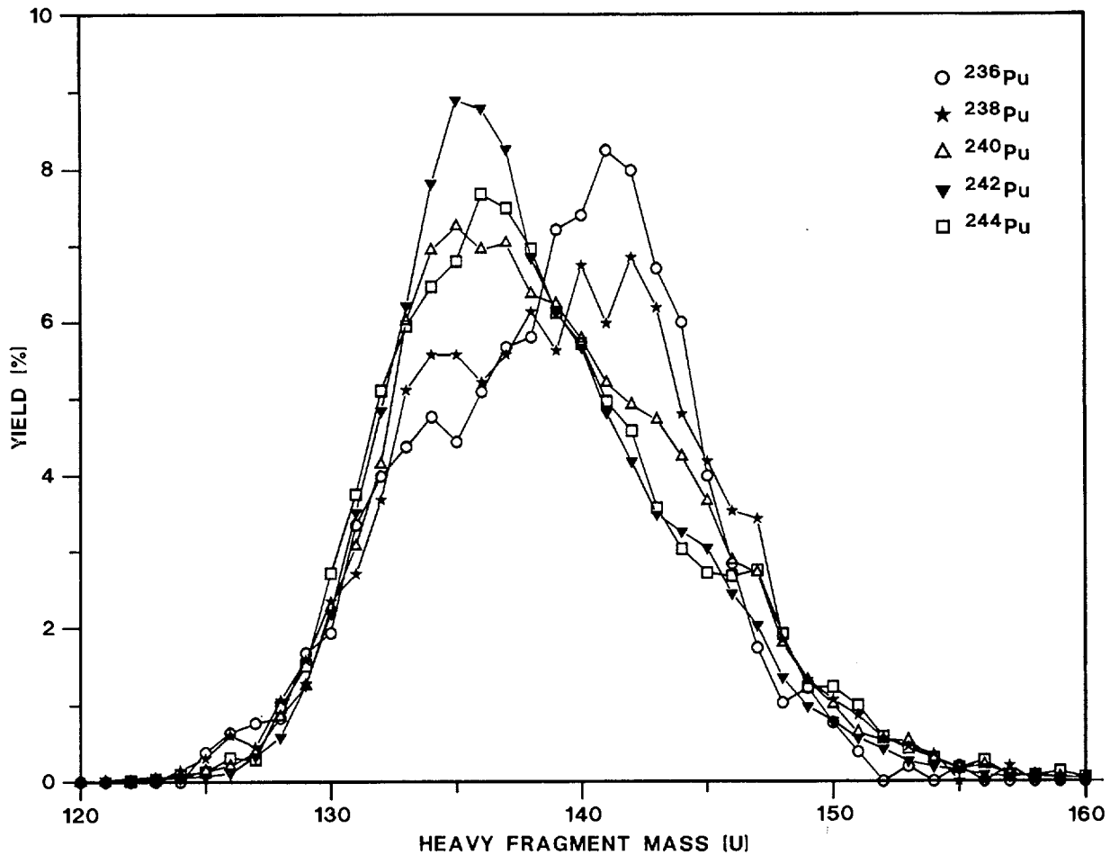
Fig. 12. Comparison of the pre-neutron emission mass distributions for ^{236}, ^{238}, ^{240}, ^{242}, ^{244}\text{Pu}(\text{S.F.})
