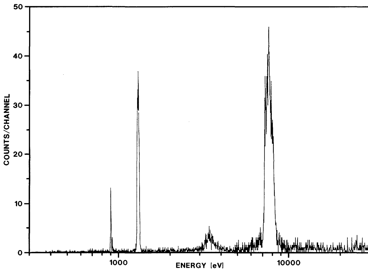
Fig. 29. ^{36}\text{Cl}(n,p) and ^{36}\text{Cl}(n,\alpha) resonances in the neutron energy region from 0.5 to 30 keV
