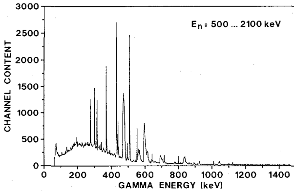
Fig. 23 Gamma-ray spectrum from the palladium sample detected within a time-of-flight window corresponding to 0.5 MeV to 2.1 MeV neutron energy
