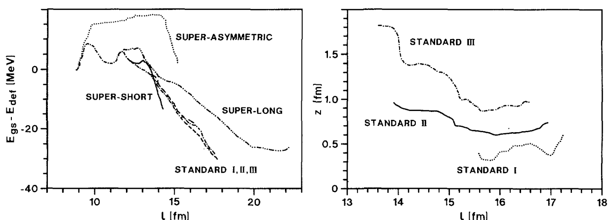
Fig. 7. Fission modes in ^{252}\text{Cf} . Left part: Potential energy E_{gs} - E_{def} of the deformed nucleus for the different fission modes as function of the elongation parameter l . Right part: Asymmetry parameter z versus elongation parameter l , shown zoomed in l between 13 fm and 18 fm to make the subsplitting into the three standard modes better visible
