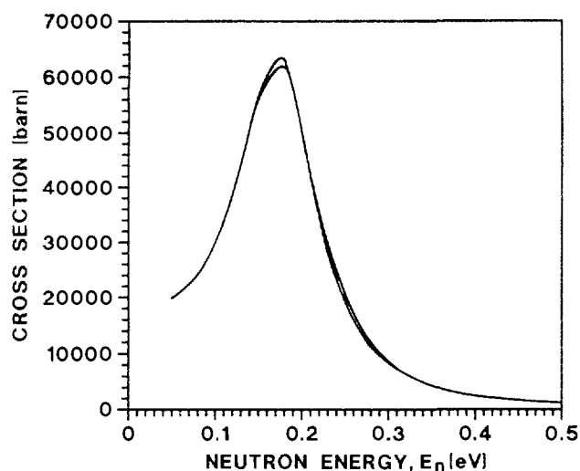
Fig. 26. The capture cross-section in the vicinity of the 0.18 eV resonance of ^{113}\text{Cd} as given by the Breit-Wigner formula and accounting for Doppler broadening at 300K
