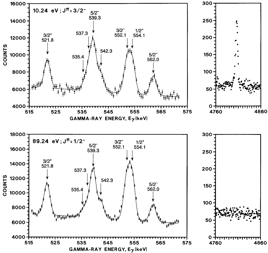
Fig. 20. Two examples of a fit of the capture gamma-ray spectrum in the 515 - 575 keV energy region for two p -waves of different spin. On the right is shown the region around the 4806 keV transition to the 5/2^+ ground state, observed only in the p 3/2 resonance
