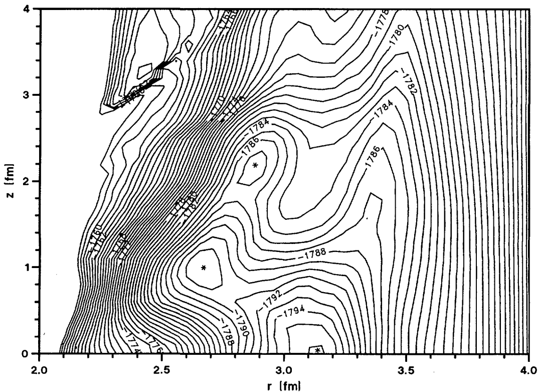
Fig. 10. Typical energy landscape in the new RAYLSCAN representation. The different fission modes are indicated by stars
