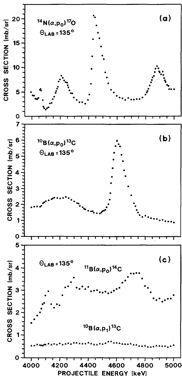
Fig. 35. Excitation functions of (a) the ^{14}\text{N}(\alpha, p_0)^{17}\text{O} , (b) the ^{10}\text{B}(\alpha, p_0)^{13}\text{C} and (c) the ^{11}\text{B}(\alpha, p_0)^{14}\text{C} and ^{10}\text{B}(\alpha, p_1)^{13}\text{C} reactions respectively measured at a laboratory scattering angle \Theta_L = 135^\circ
