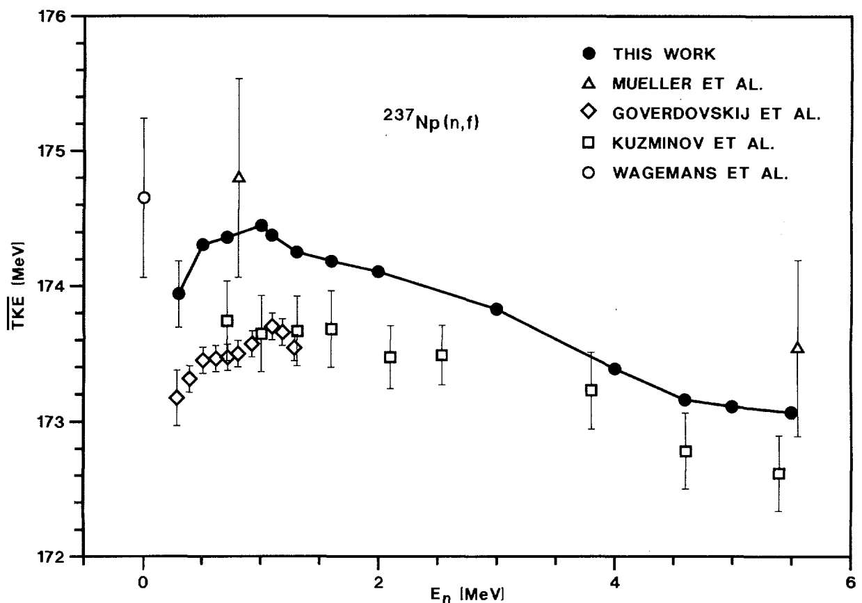
Fig. 8. Average \overline{\text{TKE}} as function of the incident neutron energy
