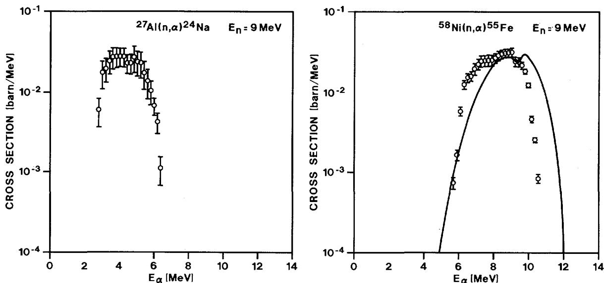
Fig. 18. The alpha particle energy spectrum for the ^{27}\text{Al}(n,\alpha) reaction at E_n = 9 MeV (left). The alpha particle energy spectrum for the ^{58}\text{Ni}(n,\alpha) reaction at E_n = 9 MeV and a calculated spectrum (STAPRE) (right)
