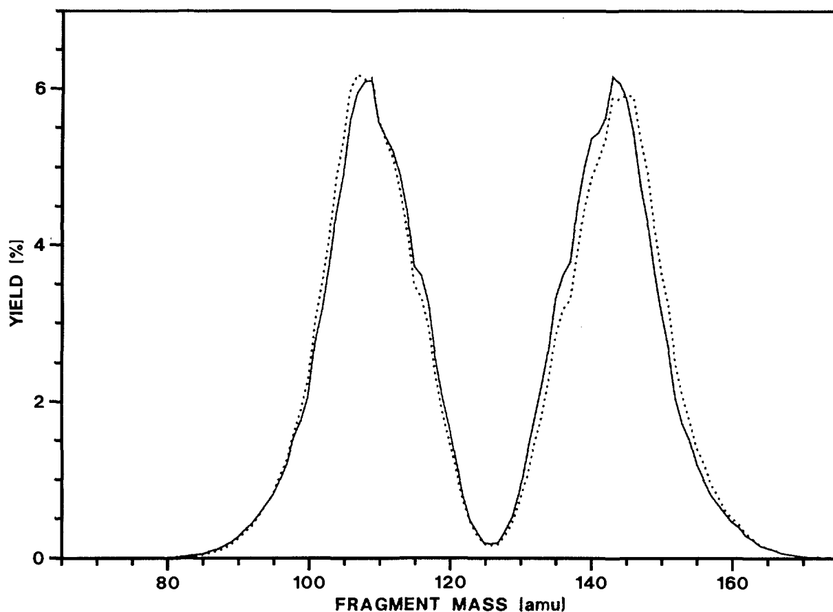
Fig. 6. Comparison of the preneutron mass distribution for methane at different pressure 1.2 \cdot 10^5 Pa (dotted line), 0.6 \cdot 10^5 Pa (solid line)
