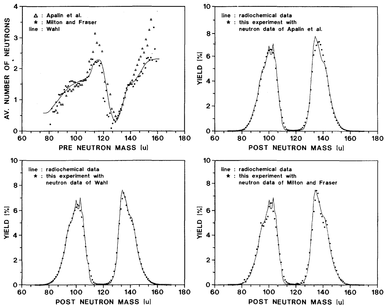
Fig. 11. \langle \nu \rangle(m_i^*) data for ^{239}\text{Pu} ( n_{th}, f ) used in the correction procedure (upper left). The corresponding post-neutron mass distributions are compared with the radiochemical data compiled by Wahl
