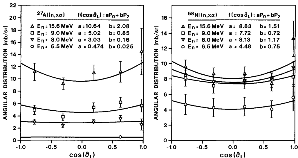
Fig. 17. Measured angular distributions and analytical fit of the ^{27}\text{Al}(n,\alpha) reaction (left). Measured angular distributions and analytical fit of the ^{58}\text{Ni}(n,\alpha) reaction (right)
