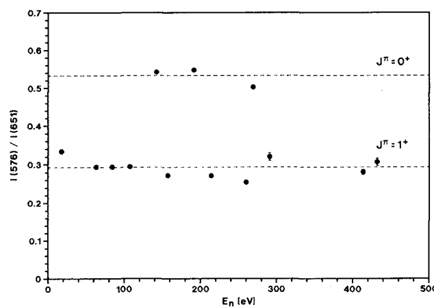
Fig. 22. The ratio of two suitable transitions, splitting up into two groups according to the spin. The error bars are within the plot symbols
