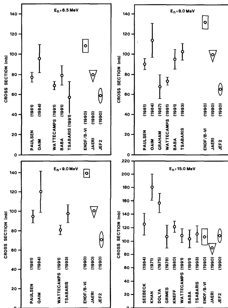
Fig. 19. Summary of total alpha particle yields of the ^{58}\text{Ni}(n,\alpha) reaction at various neutron energies
