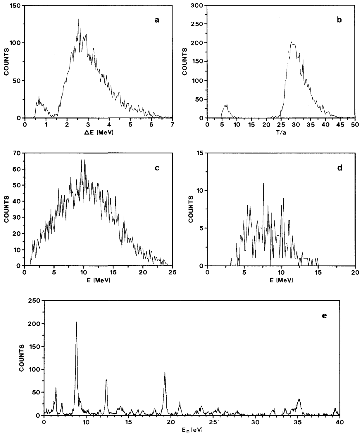
Fig. 13. Measurements on ternary fission in ^{235}\text{U}(n,f) . (a) \Delta E -spectrum of \alpha -particles and tritons (b) identification spectrum of the ternary particles T/a=(E-\Delta E)1.73-(E)1.73 , (c) energy deposited in the surface barrier detector by the \alpha -particles, (d) E -spectrum of the tritons, (e) ternary fission cross-section of ^{235}\text{U} as a function of the incident neutron energy
