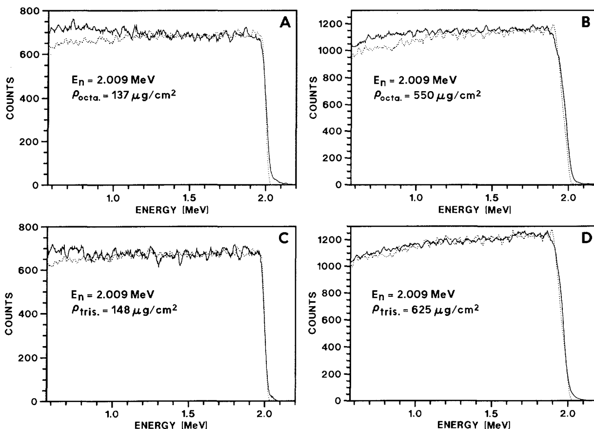
Fig. 4. Comparison of the proton recoil spectra calculated with the Monte-Carlo method (dotted line) and the experiment (solid line): (A) thinnest octacosanol sample, (B) thickest octacosanol sample, (C) thinnest tristearin sample and (D) thickest tristearin sample, all at about 2 MeV incident neutron energy
