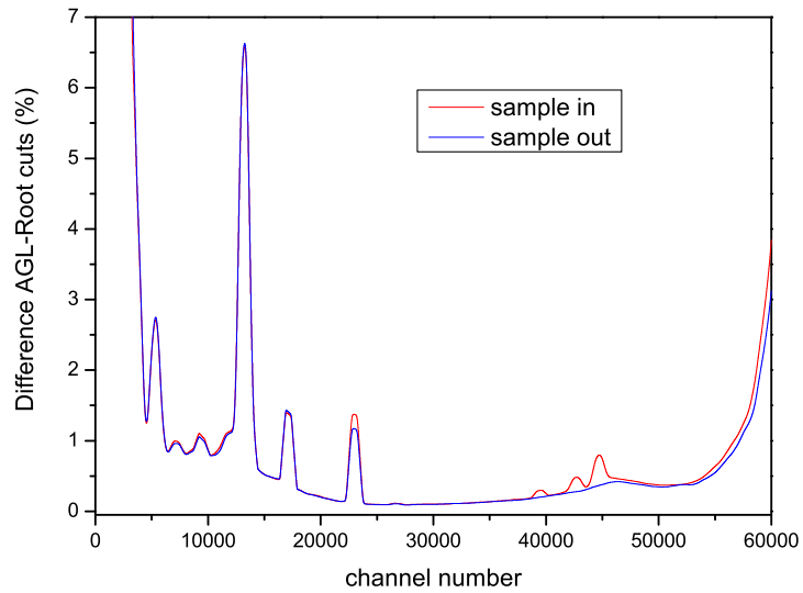
Figure 6.7: Relative difference (AGL-Root)/AGL in % between the AGL and Root cuts in the reconstructed TOF spectra regrouped per 500 channels.
