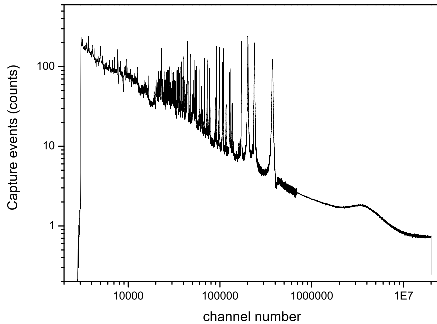
Figure 7.7: Raw 241 Am(n,γ) data from one of the C 6 D 6 detectors.
