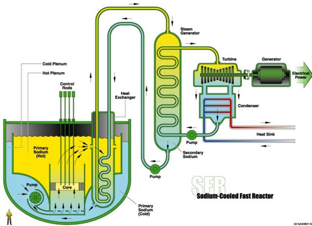
Figure 1.4: Scheme of the Sodium cooled Fast Reactor (SFR) concept [4].
