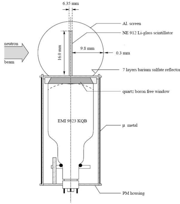
Figure 5.7: Scheme of a 0.25" thick Li-glass detector coupled with a photomultiplier.
