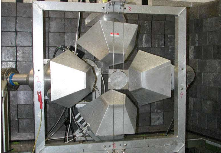
Figure 7.5: Picture of the 4 detectors setup.
