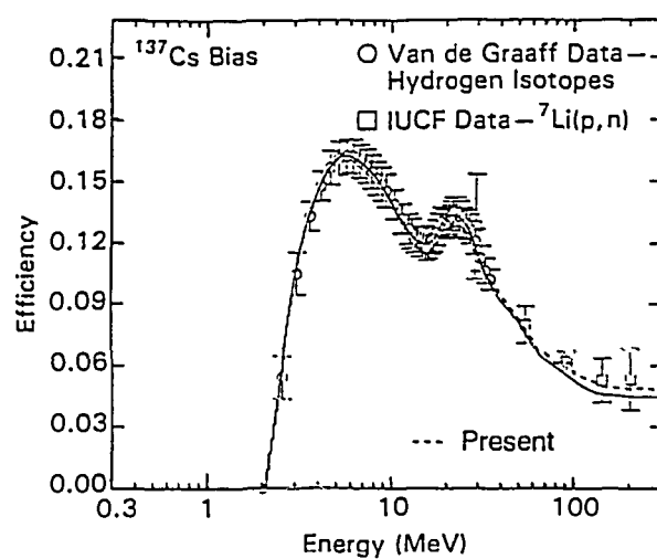
Fig. 6 Neutron detection efficiency used in the TOF technique compared with the values measured at IUCF.
