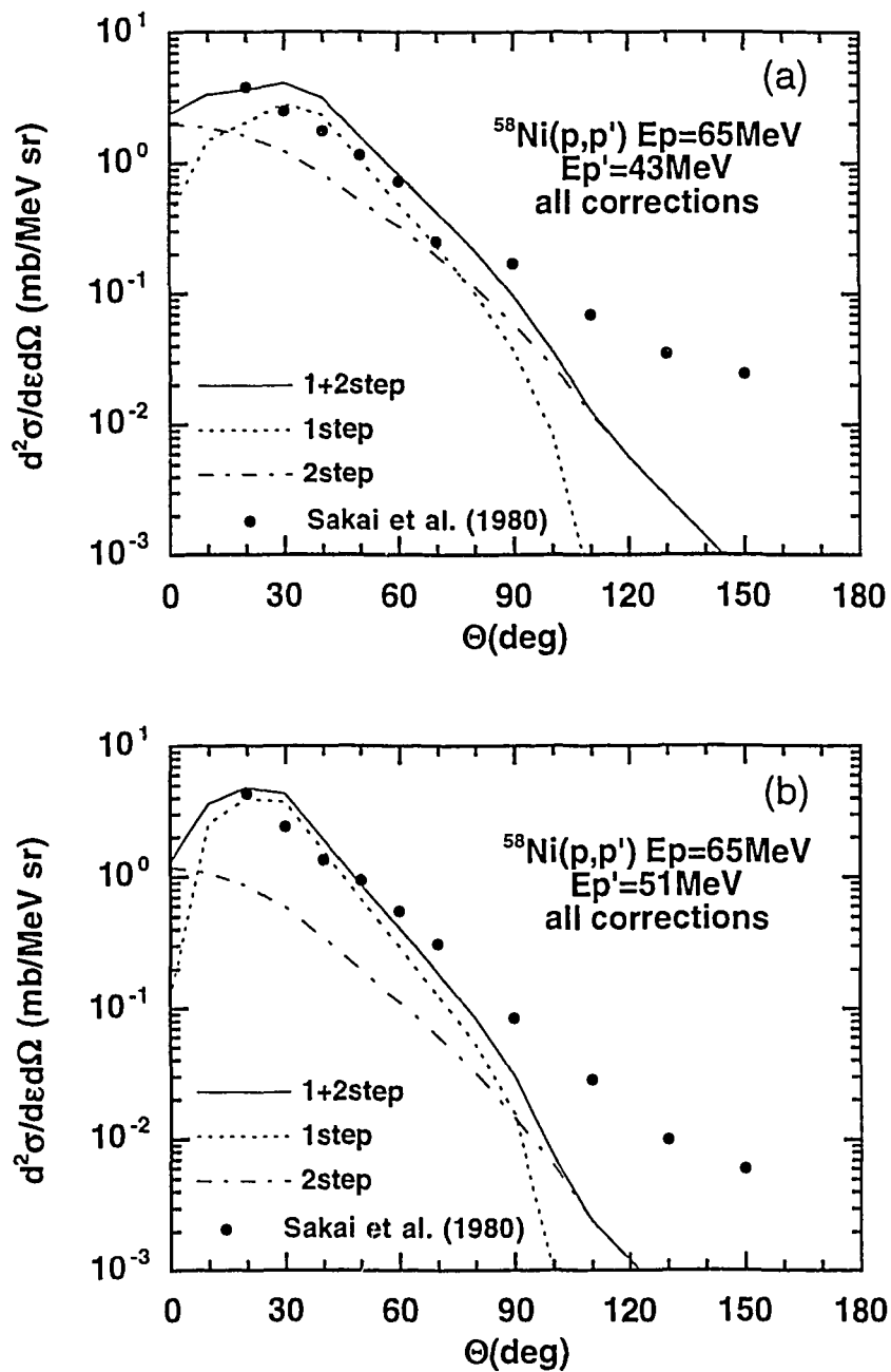
Fig.4 Angular distribution of ^{58}\text{Ni}(p,p')x at 65 MeV for outgoing energies of (a) 43 MeV and (b) 51 MeV. The closed circles are experimental data taken from ref. [19]. Also, see Fig.3 for the explanation of each line.
