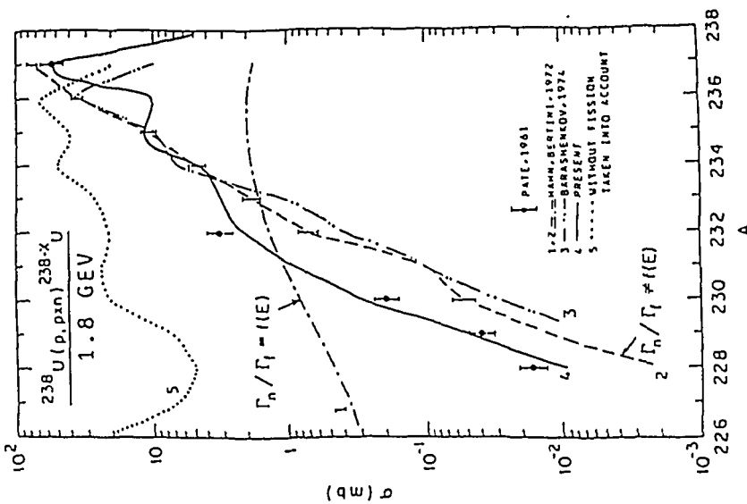
Fig. 7. The yield of uranium isotopes in the reaction ^{238}\text{U}(\text{p},\text{pxn})^{238-\text{x}}\text{U} at 1.8 GeV.
