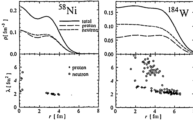
FIG. 11. Density distribution (upper parts) and Gaussian widths (lower parts) of ^{58}\text{Ni} and ^{184}\text{W} nuclei. Horizontal axes for both denote the distance from the center.
