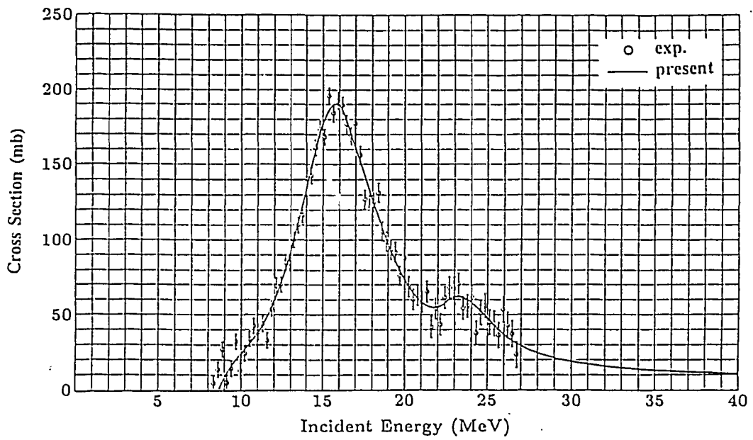
Fig. 5 The (\gamma, xn) cross section of ^{98}\text{Mo} .
