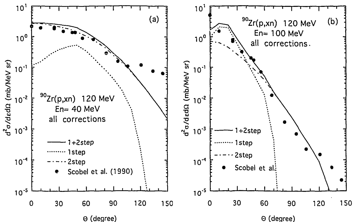
Fig.6 Angular distribution of ^{90}\text{Zr}(p,xn) at 120 MeV for outgoing energies of (a) E_n=40 \text{ MeV} and (b) 100 MeV. The dotted and dash-dotted lines present the one-step and the two-step SCDW calculations, respectively. The solid line is their sum. The experimental data are taken from ref. [22].
