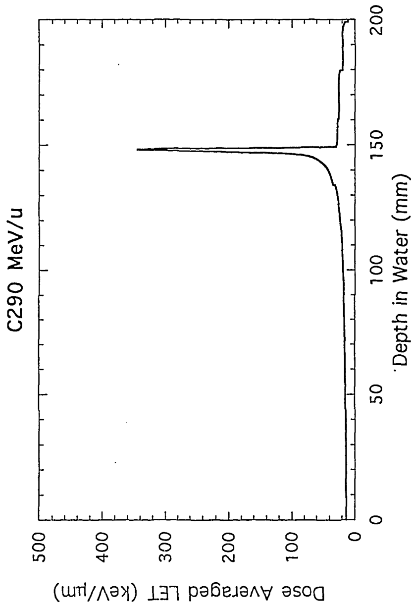
Fig. 3 the calculated LET distribution of the 290 MeV/u carbon beam in water material.
