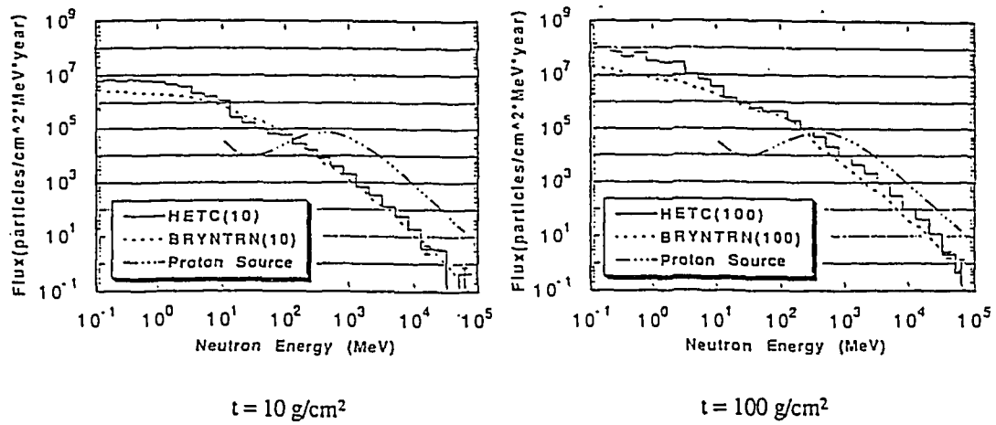
Fig.10 Calculated neutron spectra by BRYNTRN and HETC-MCNP.
