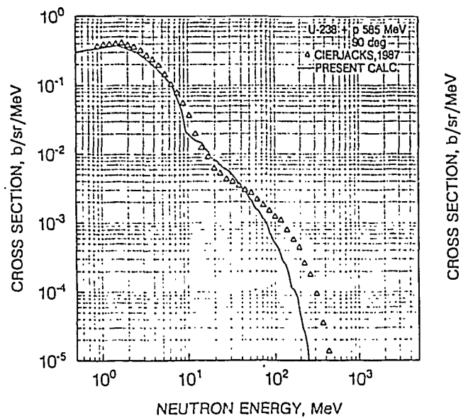
Fig. 12 Comparison of the present calculations of double differential neutron production cross sections for ^{238}\text{U} at E_p = 585 MeV and 90^\circ deg with experimental data [45].
