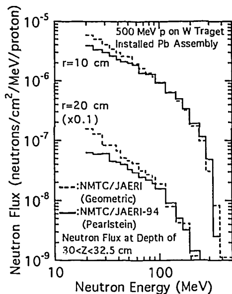
Fig. 3 Calculated neutron energy spectra at the depth between 30 and 32.5 cm in the radial distance of 10 and 20 cm for 500 MeV proton incidence on tungsten target installed lead assembly having the size of 60 cm in diameter and 100 cm in length.
