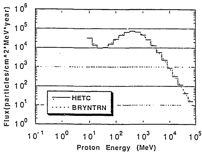
Fig.8 Incident proton spectra.
