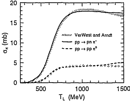
FIG. 2. Pion production cross section.
