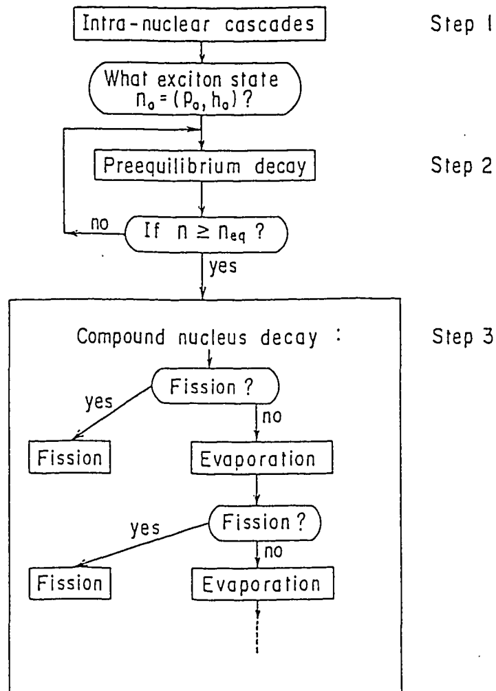
Fig.1 Three-step simulation scheme of the hadron induced nuclear reactions in the intermediate energy region
