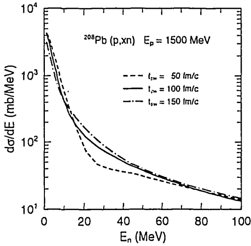
FIG. 8. Neutron spectra in p (1.5 GeV) + ^{208}\text{Pb} reaction, comparing the results for switching time t_{\text{sw}} at 50, 100 and 150 fm/c.
