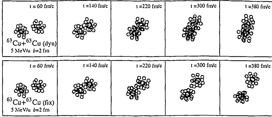
FIG. 13. An example of ^{63}\text{Cu} + ^{63}\text{Cu} (5 MeV/u) reaction. Upper part shows full EQMD calculation of 8N -dimensional equation of motion, while the lower part shows 6N -dimensional constrained calculation with fixed width.
