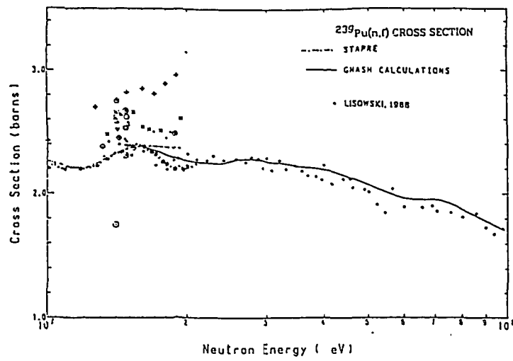
Fig. 4. The ^{239}\text{Pu} fission cross section.
