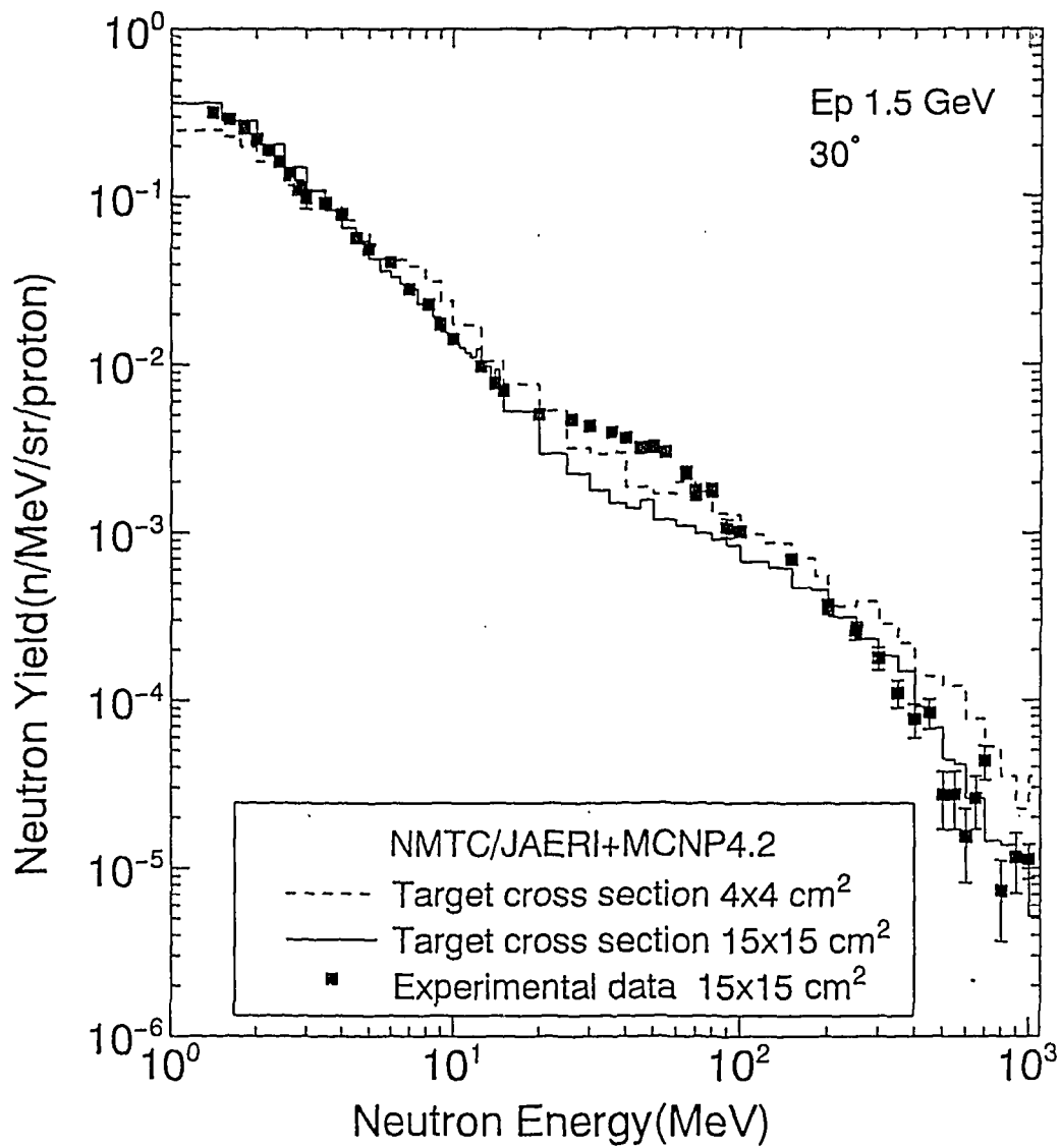
Fig. 13 Calculation result of neutron spectra from small target (4x4x20 cm 2 ) and present target compared with the experimental data.
