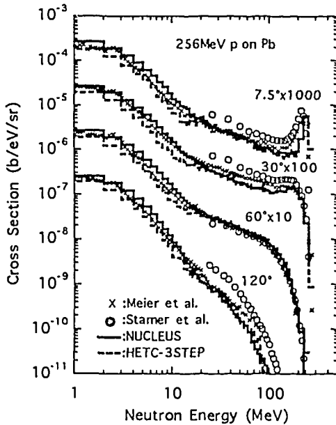
Fig. 11 Experimental and calculated neutron differential cross sections of ^{208}\text{Pb} for 256 MeV proton incidence. The solid, and the dotted lines indicate the results of NUCLEUS and HETC-3STEP, respectively.
