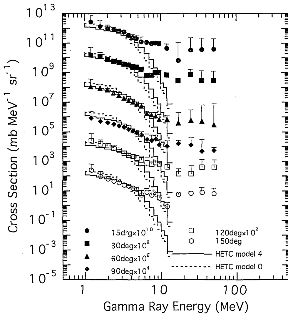
Fig. 12 Gamma ray production double differential cross section for 0.8 GeV p on Pb.
