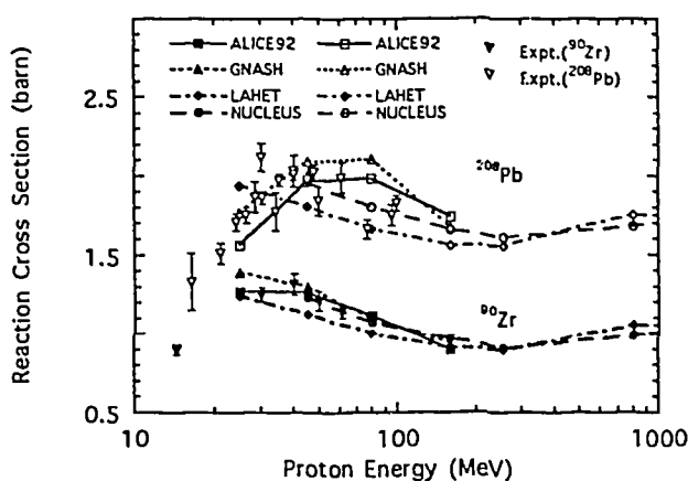
Fig. 1 Total reaction cross sections calculated with the codes ALICE92, GNASH, LAHET and NUCLEUS for proton incidence on ^{90}\text{Zr} and ^{208}\text{Pb} .
