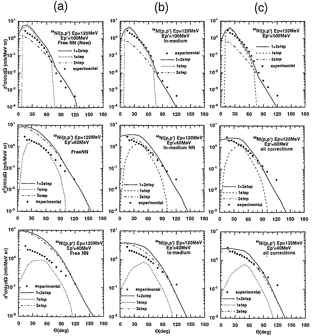
Fig.2 Comparisons of the SCDW calculation and the experimental data for ^{58}\text{Ni}(p,p')x at 120 MeV. The dotted and the dash-dotted lines present the one-step and the two-step SCDW calculations, respectively, and the solid line is their sum. (a) The case with the free NN cross section. (b) The case with the in-medium NN cross section and (c) The case where the nonlocality correction is taken into account for the struck nucleon in addition to the calculation of (b). See the details in text. The experimental data are taken from ref. [18].
