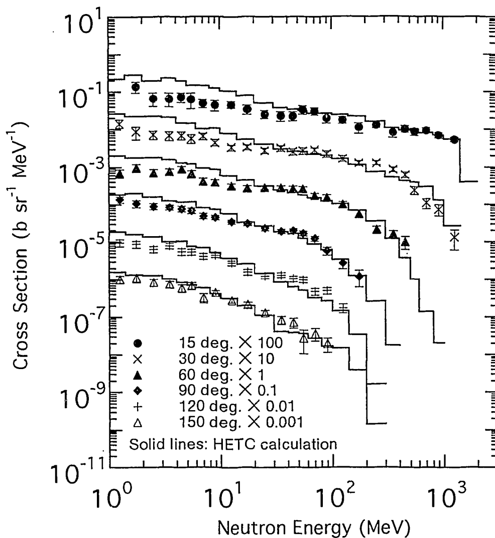
Fig. 6 Neutron production double differential cross section for 1.5 GeV p on C.
