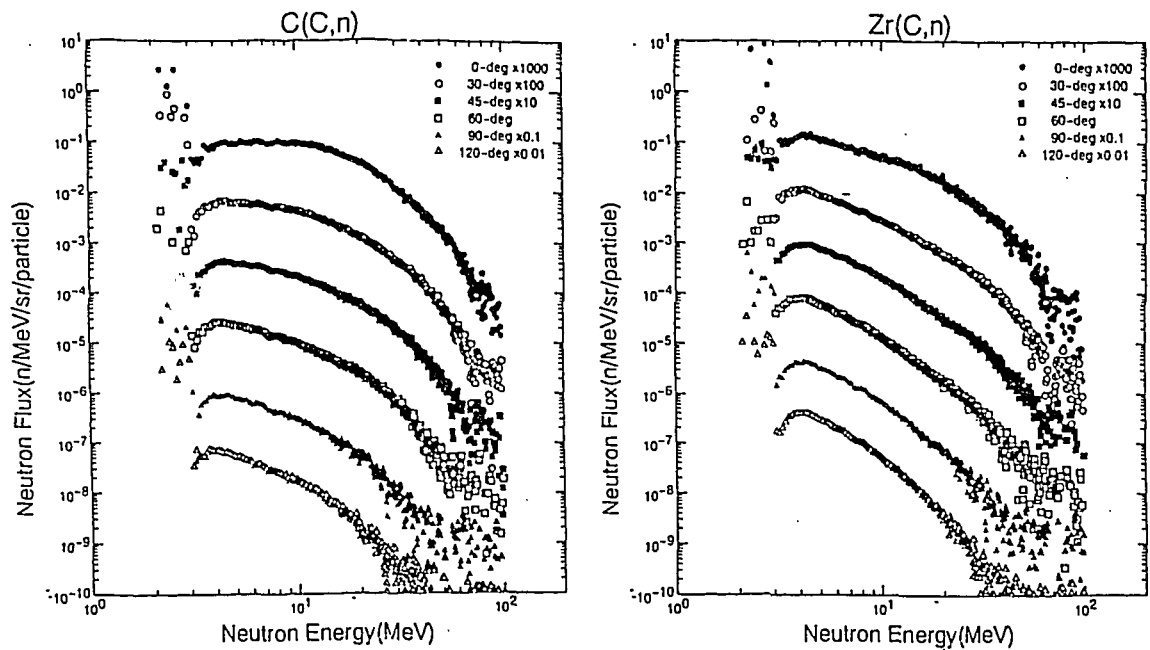
Fig. 8 Differential neutron spectra for C and Zr targets bombarded by 220 MeV C ions
