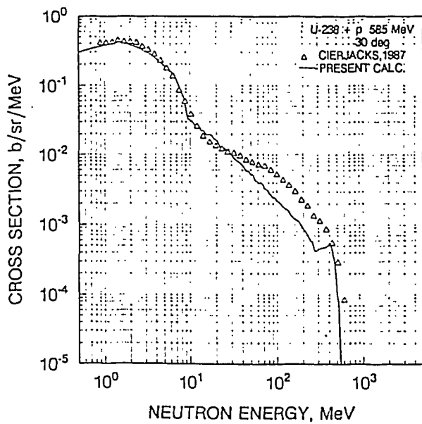
Fig. 11 Comparison of the present calculations of double differential neutron production cross sections for ^{238}\text{U} at E_p = 585 MeV and 30^\circ deg with experimental data [45].
