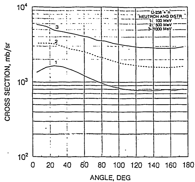
Fig. 10. Neutron angular distributions for ^{238}\text{U} neutron bombardment with energies of 100, 500 and 1000 MeV.
