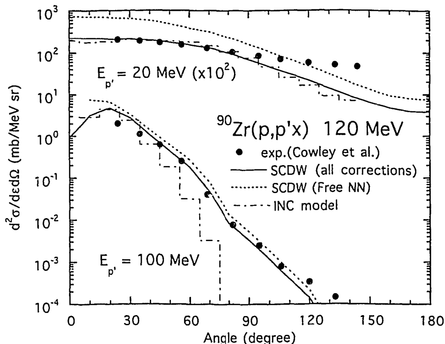
Fig.5 Angular distribution of ^{90}\text{Zr}(p,p'x) at 120 MeV for outgoing energies of E_{p'}=20 \text{ MeV} and 100 MeV. The solid and dotted lines present the SCDW calculations with all corrections (see in Fig.1(c)) and with the Free N-N cross section (see in Fig.1(a)), respectively. The dash-dotted histogram denotes the INC model calculation. The data are taken from ref. [20].
