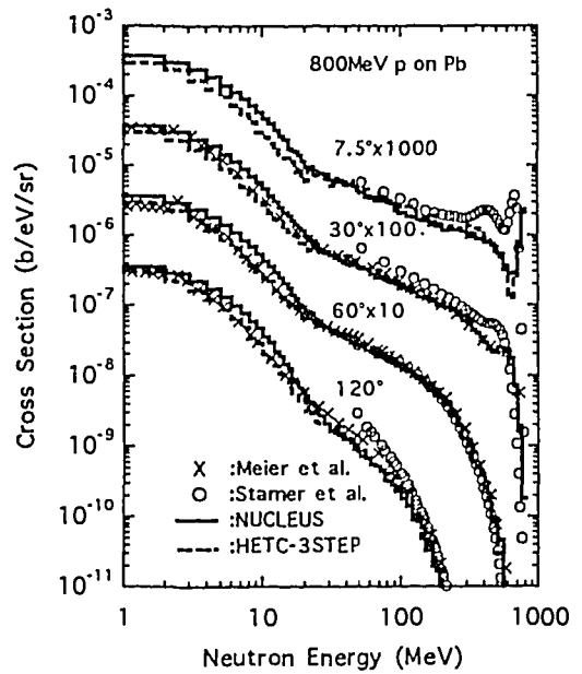
Fig. 12 Experimental and calculated neutron differential cross sections of ^{208}\text{Pb} for 800 MeV proton incidence. The solid, and the dotted lines indicate the results of NUCLEUS and HETC-3STEP, respectively.
