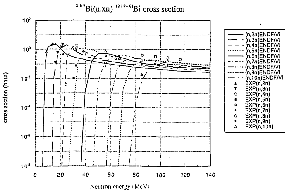
Fig.14 Cross section data of ^{209}Bi(n,xn) reaction compared with ENDF/B-VI
