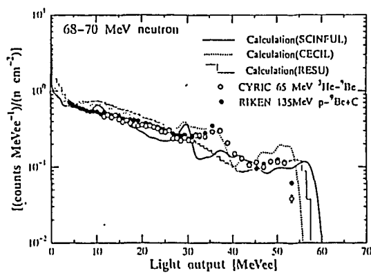
Fig. 7 Measured and calculated response functions of 12.7 cm diam by 12.7 cm long BC501A scintillator for 29 to 30 MeV and 68 to 70 MeV neutrons
