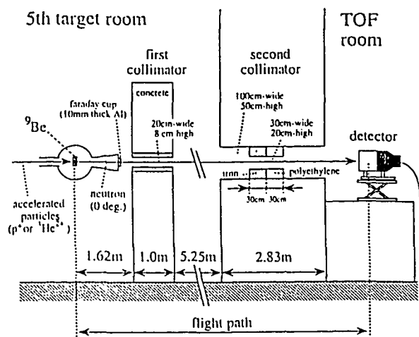
Fig. 1 Cross-sectional view of the CYRIC neutron field
