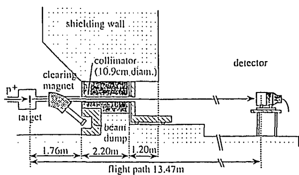
Fig. 3 Cross-sectional view of the TIARA neutron field
