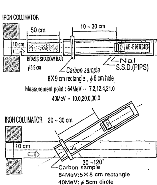
Fig. 9 Experimental arrangement with the proton recoil counter telescope
