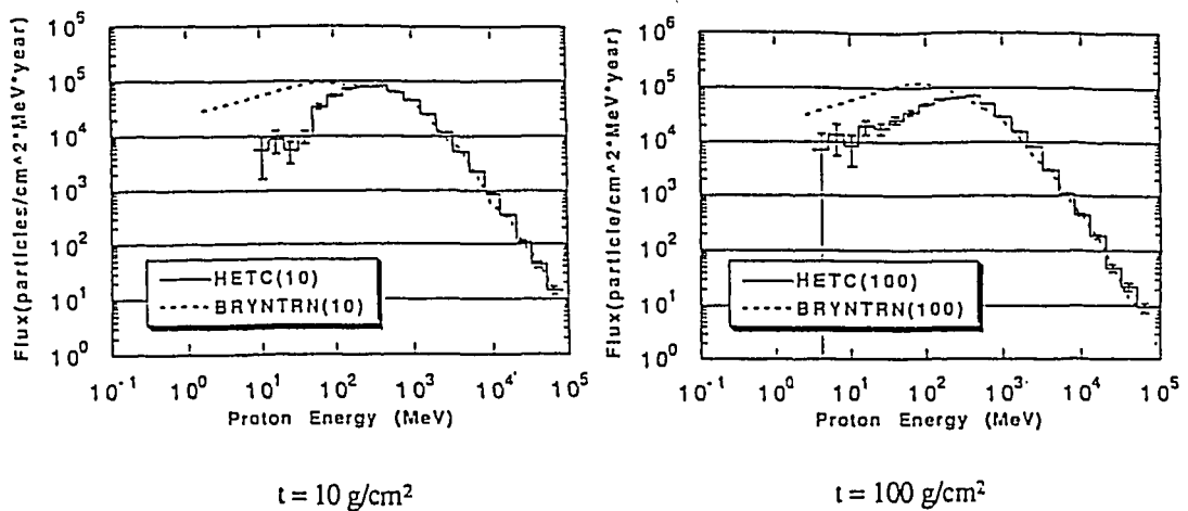
Fig.9 Calculated proton spectra by BRYNTRN and HETC-MCNP.
