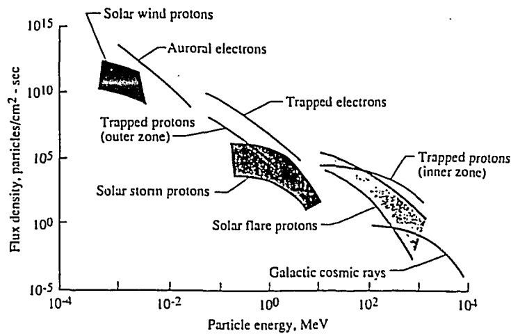
Fig.1 Space-radiation environment.
