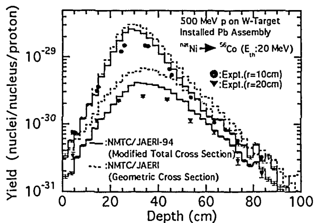
Fig. 4 Experimental and calculated yields of ^{56}\text{Co} in ^{\text{nat}}\text{Ni} samples inserted into tungsten target installed lead assembly for 500 MeV proton bombardment. Solid lines represent the calculated results of NMTC/JAERI with the total cross section evaluated by Pearlstein. Dashed lines denote the calculated results using geometric cross section.
