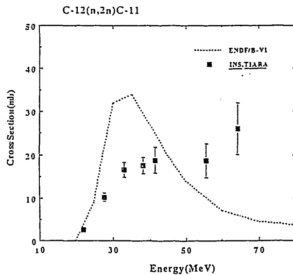
Fig.13 Cross section data of ^{12}C(n,2n) reaction compared with ENDF/B-VI
