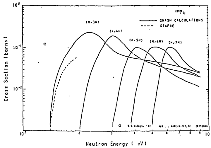
Fig. 5. The ^{239}\text{Pu}(n,xn) reaction cross sections.
