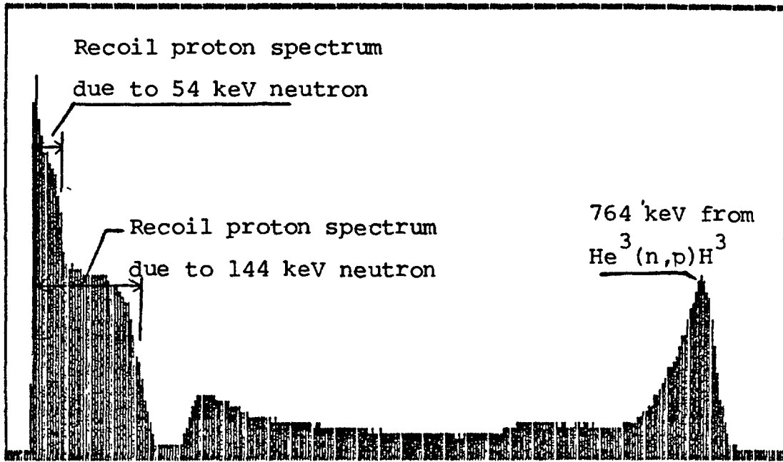
Fig. 2 . Total energy spectrum from recoil proton detector.
