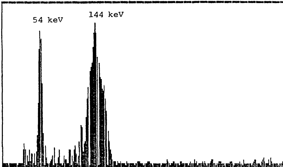
Fig. 3 . Neutron beam differential spectrum.
