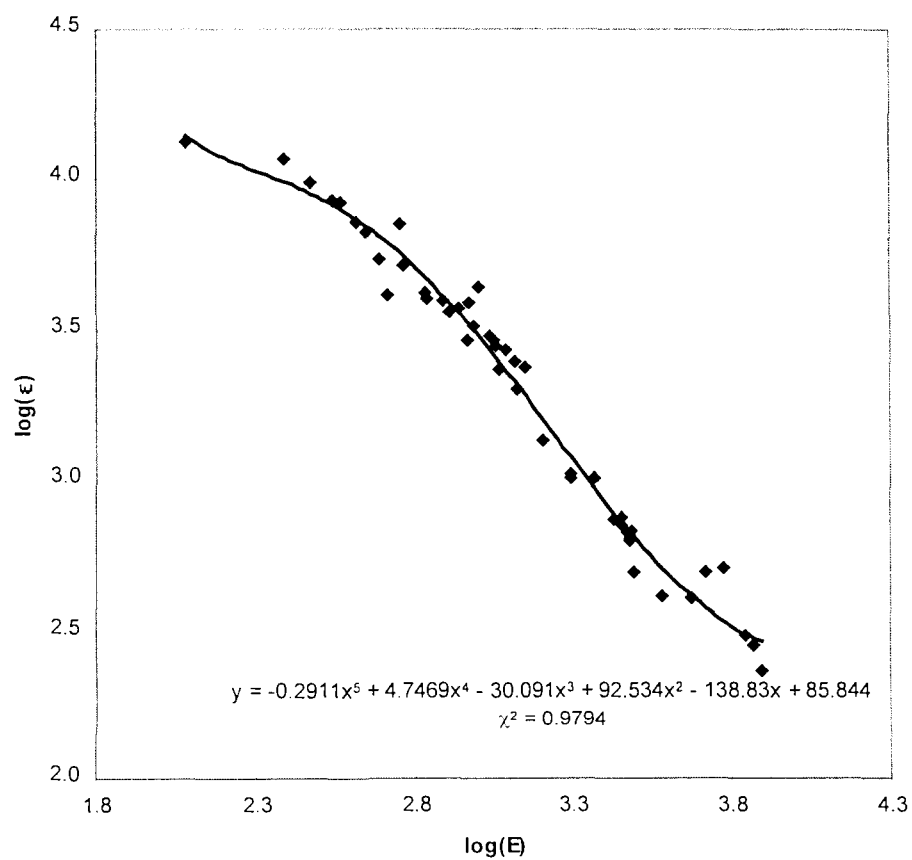
Fig.4: Relative efficiency curve of the spectrometer
