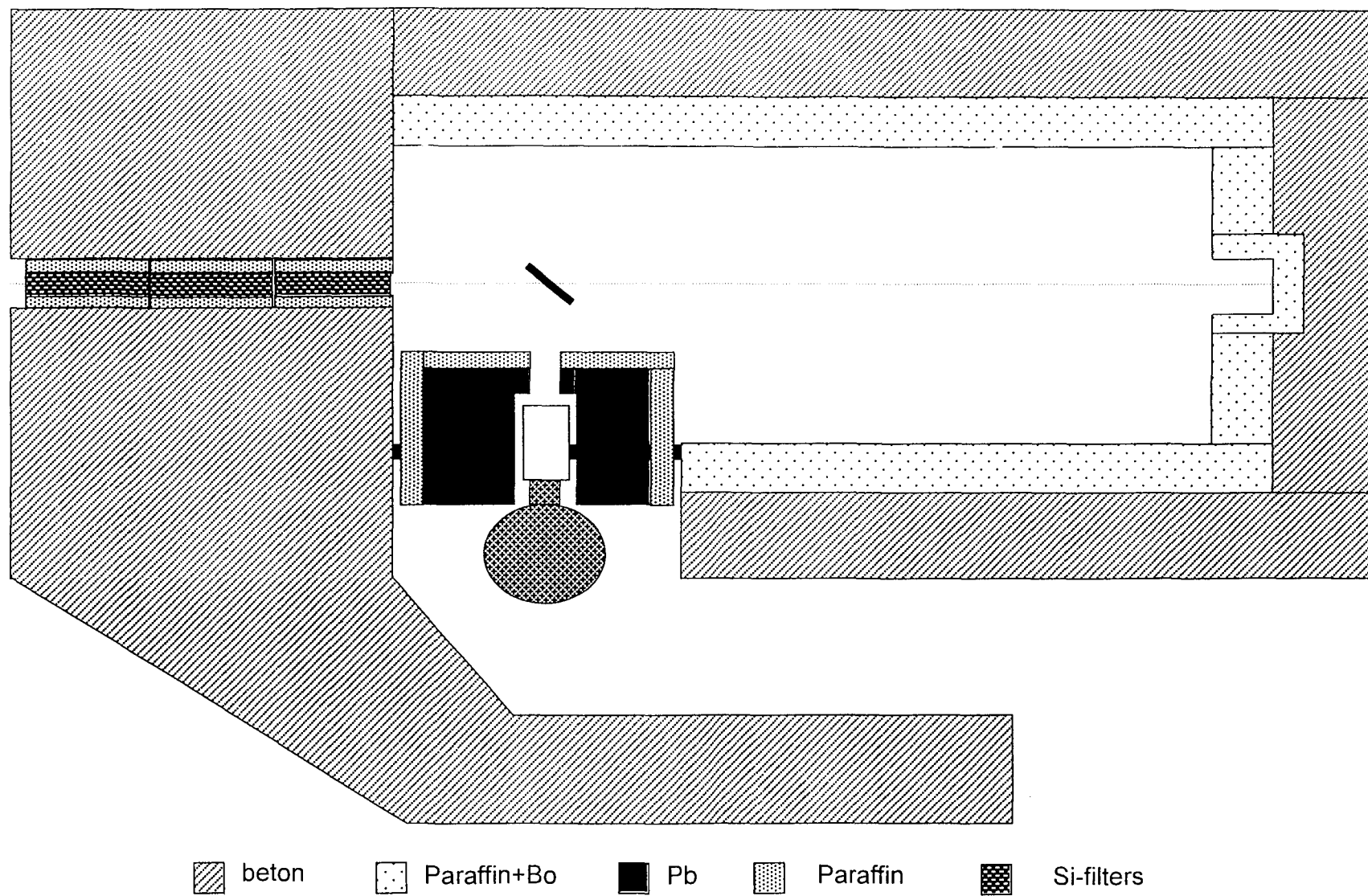
Fig.2: Sectional view of the lay-out of the shield and arrangement of instruments
