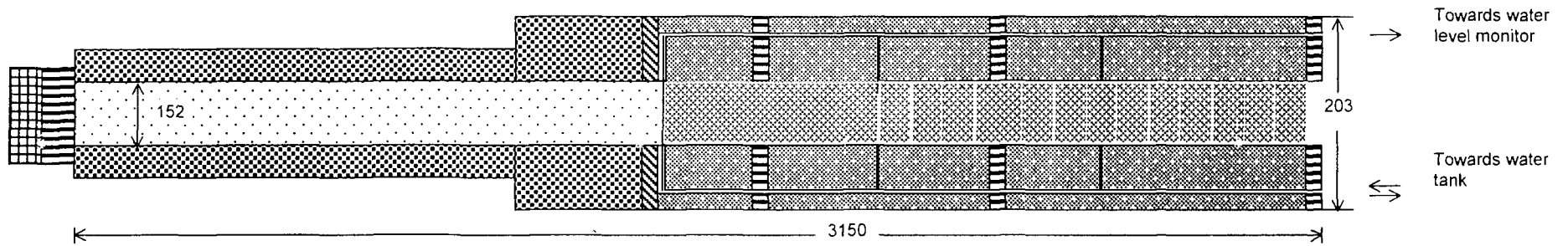
Fig.3: Sectional view of the tangential beam tube
