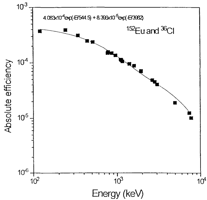
Fig. 1: Absolute efficiency vs. Energy of Gamma-ray
