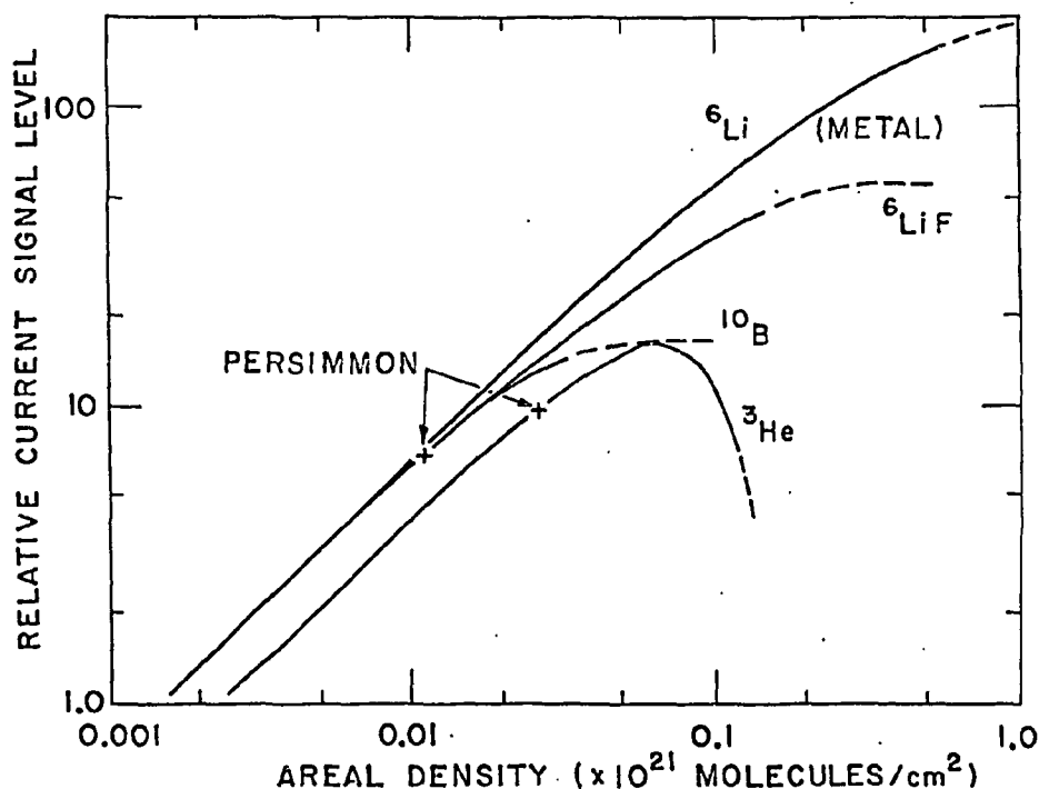
Fig. 4. Comparison of alternative materials for flux measurement at low neutron energies, in terms of relative signal level vs areal density of the target material.
