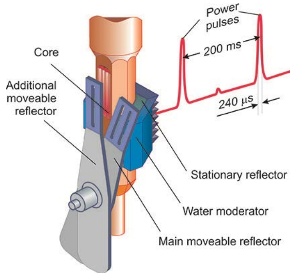
FIG.3. Schematic picture of IBR-2 pulsed reactor [5]
