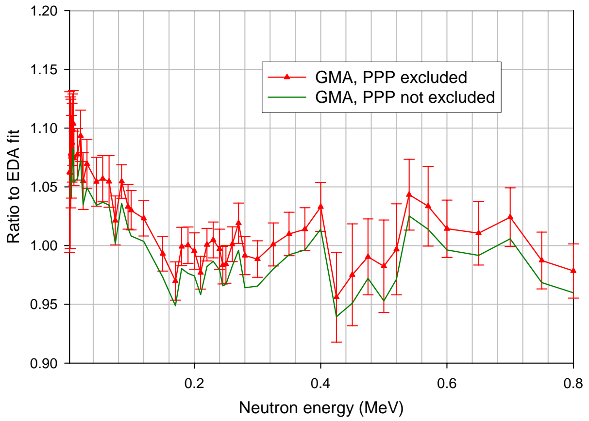
{}^6\text{Li}(n,t) comparison for TEST2
