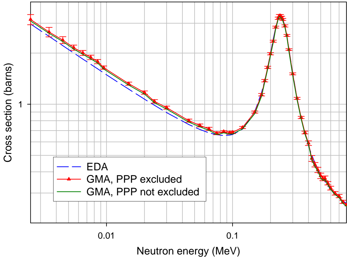
{}^6\text{Li}(n,t) comparison for TEST2
