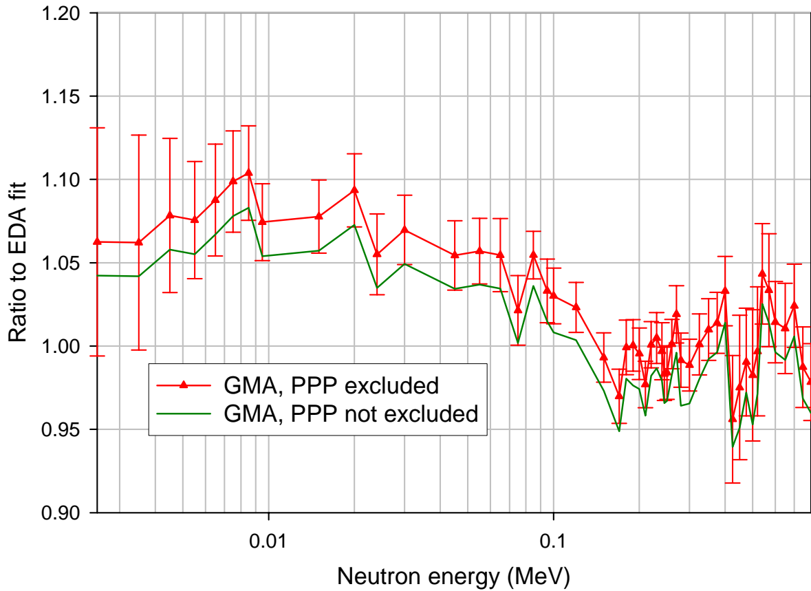
{}^6\text{Li}(n,t) comparison for TEST2
