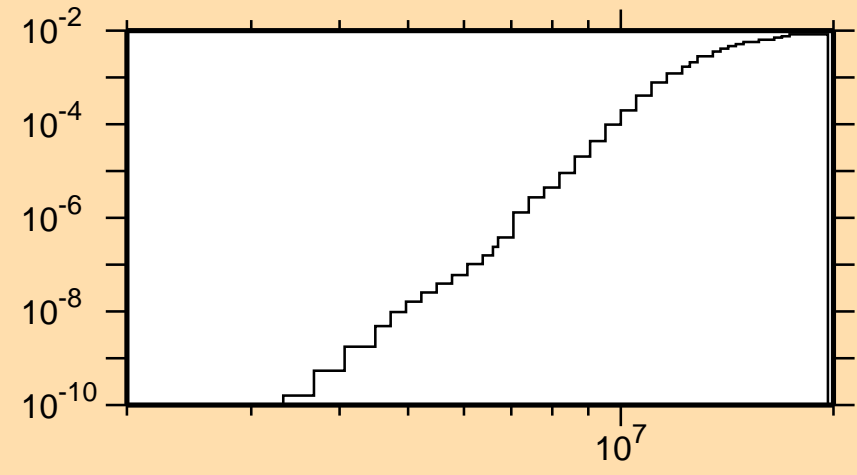
\sigma vs. E for ^{183}\text{W}(\text{mt855})
