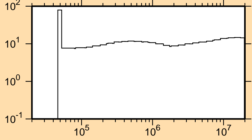
\Delta\sigma/\sigma vs. E for ^{183}\text{W}(n,n_1)
