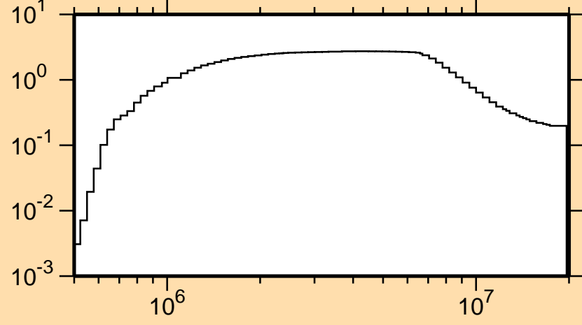
\sigma vs. E for ^{183}\text{W}(\text{mt854})
