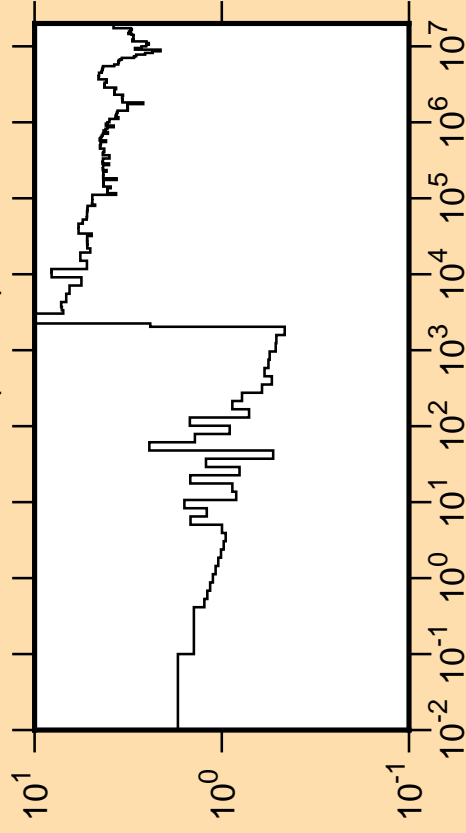
\Delta\sigma/\sigma vs. E for ^{183}\text{W}(n,\text{tot.})
