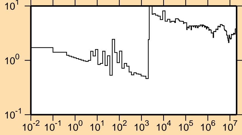
\Delta\sigma/\sigma vs. E for ^{183}\text{W}(n,\text{tot.})
