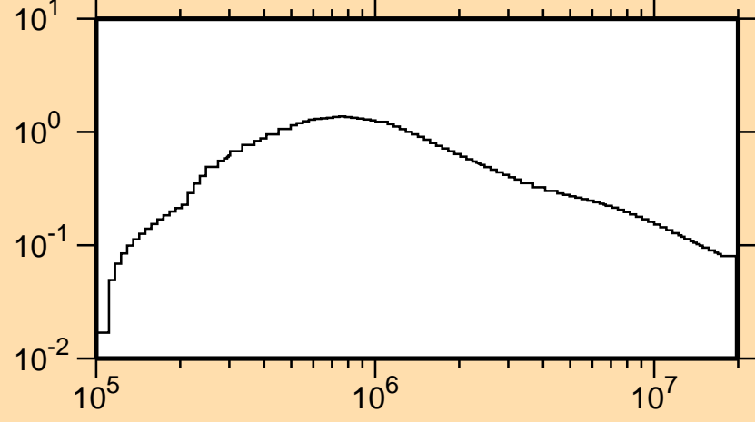
\sigma vs. E for ^{183}\text{W}(\text{mt853})
