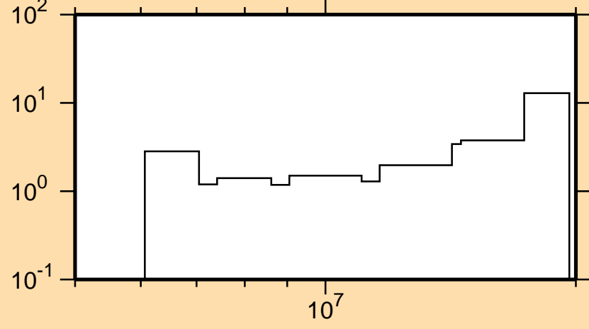
\Delta\sigma/\sigma vs. E for ^{183}\text{W}(\text{mt852})
