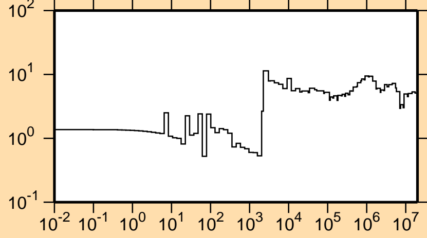
\Delta\sigma/\sigma vs. E for ^{183}\text{W}(n,\text{el.})
