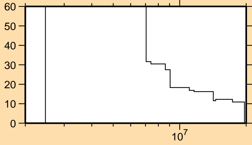
\Delta\sigma/\sigma vs. E for ^{183}\text{W}(\text{mt855})
