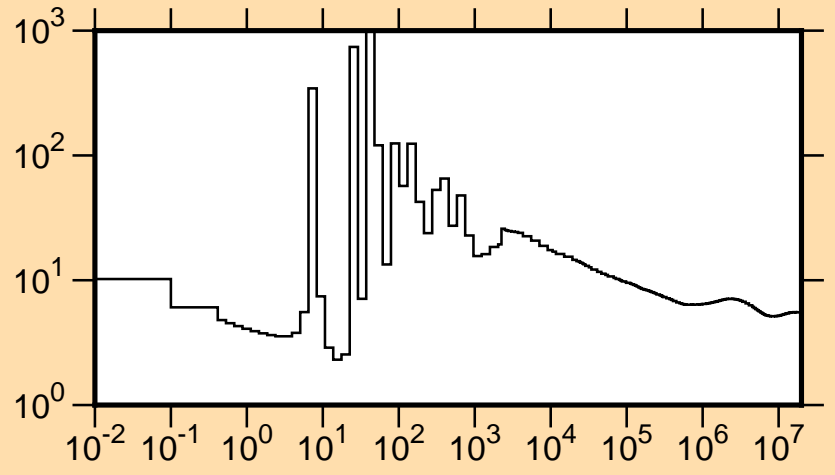
\sigma vs. E for ^{183}\text{W}(n,\text{tot.})
