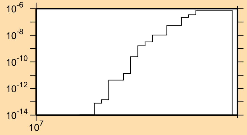
\sigma vs. E for ^{184}\text{W}(n,2n\alpha)
