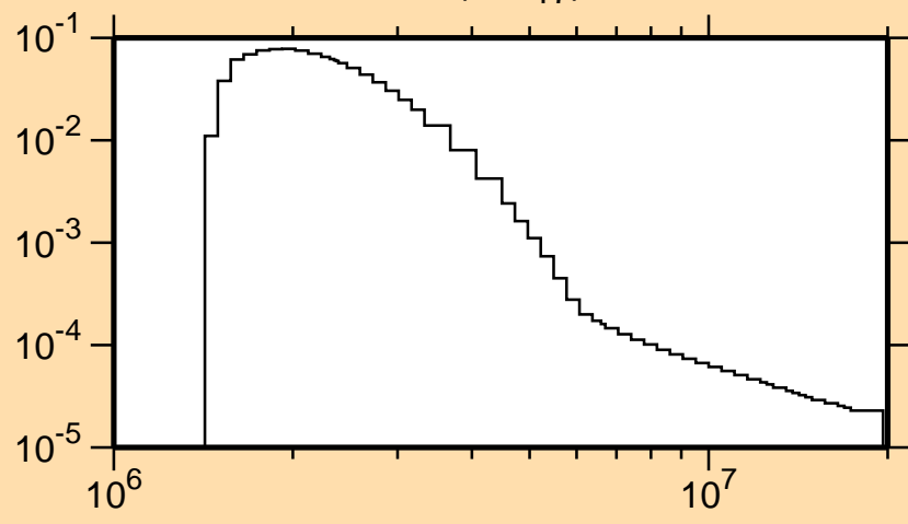
\sigma vs. E for ^{184}\text{W}(n,n_{17})
