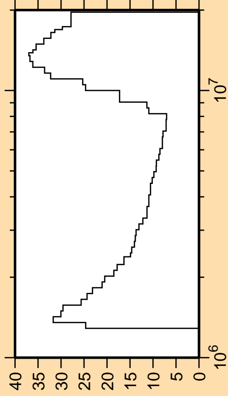
\Delta\sigma/\sigma vs. E for ^{184}\text{W}(n,n_{12})
