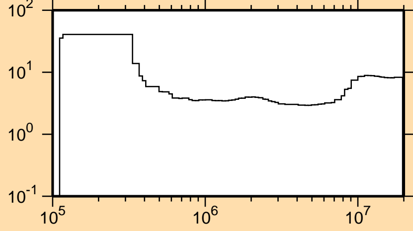
\Delta\sigma/\sigma vs. E for ^{184}\text{W}(n,n_1)
