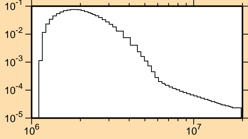
\sigma vs. E for ^{184}\text{W}(n,n_0)
