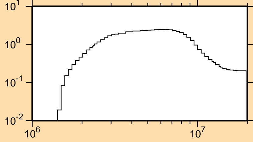
\sigma vs. E for ^{184}\text{W}(n,n\text{cont.})
