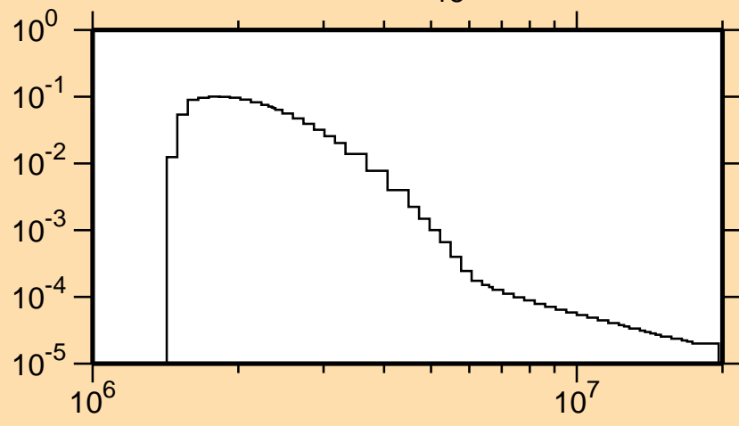
\sigma vs. E for ^{184}\text{W}(n,n_{18})
