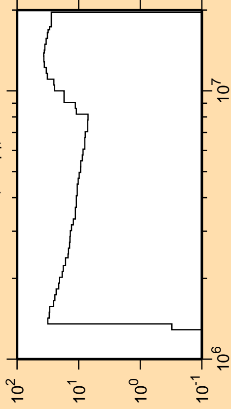
\Delta\sigma/\sigma vs. E for ^{184}\text{W}(n,n_{14})
