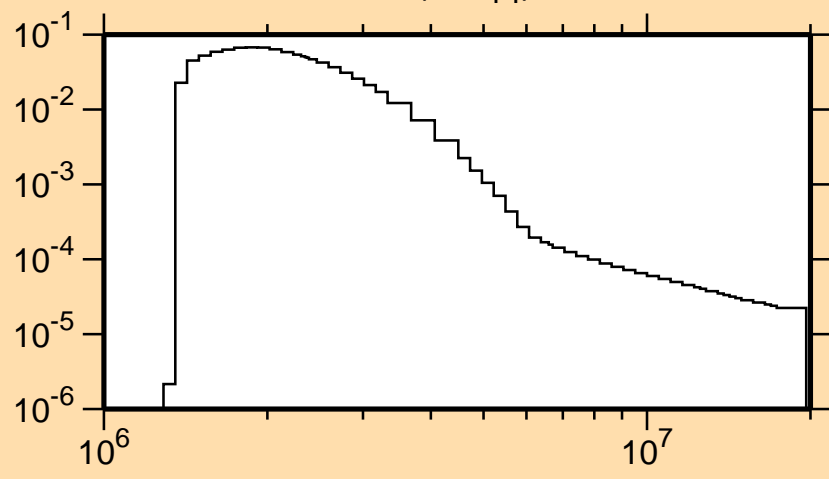
\sigma vs. E for ^{184}\text{W}(n,n_{14})
