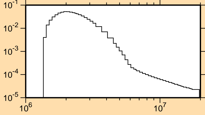
\sigma vs. E for ^{184}\text{W}(n,n_{15})
