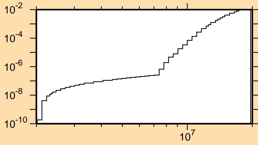
\sigma vs. E for ^{184}\text{W}(n,p)
