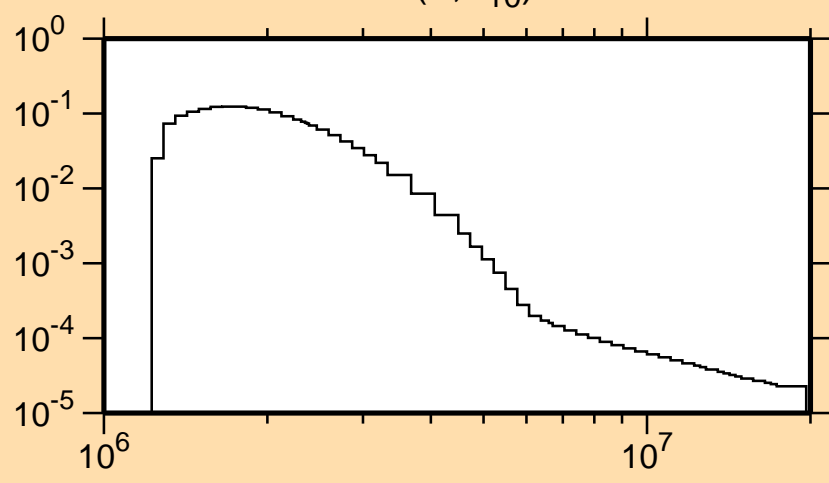
\sigma vs. E for ^{184}\text{W}(n,n_{10})
