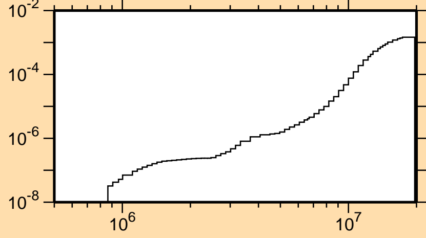
\sigma vs. E for ^{184}\text{W}(n,\alpha)
