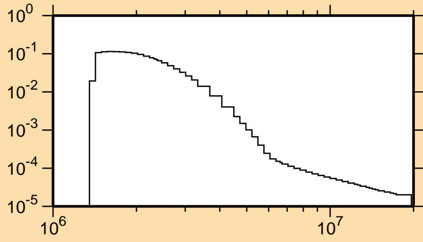
\sigma vs. E for ^{184}\text{W}(n,n_{16})
