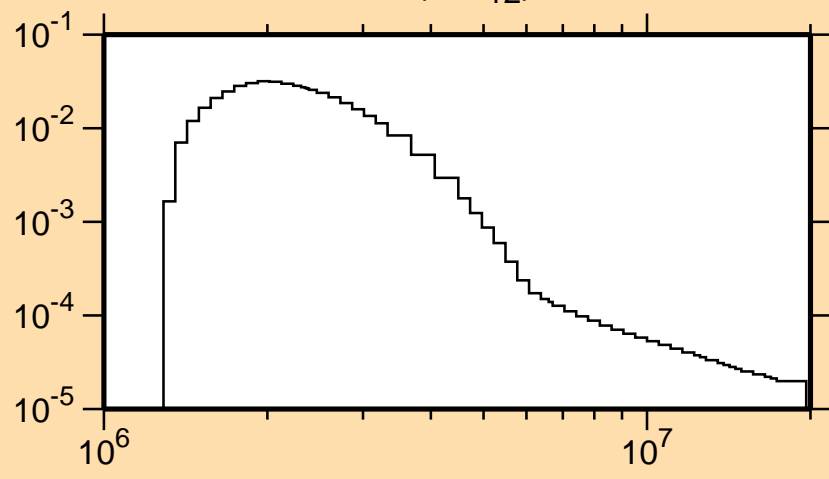
\sigma vs. E for ^{184}\text{W}(n,n_{12})
