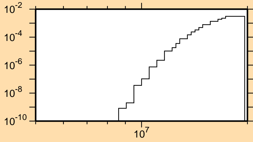
\sigma vs. E for ^{184}\text{W}(n,d)
