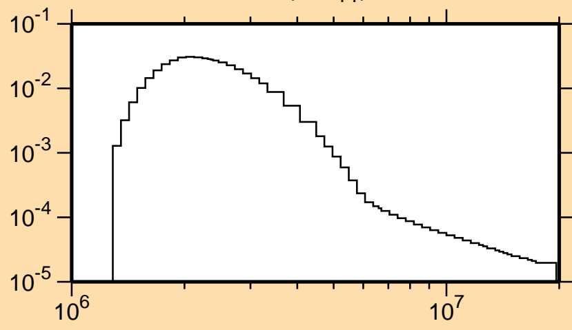
\sigma vs. E for ^{184}\text{W}(n,n_{11})
